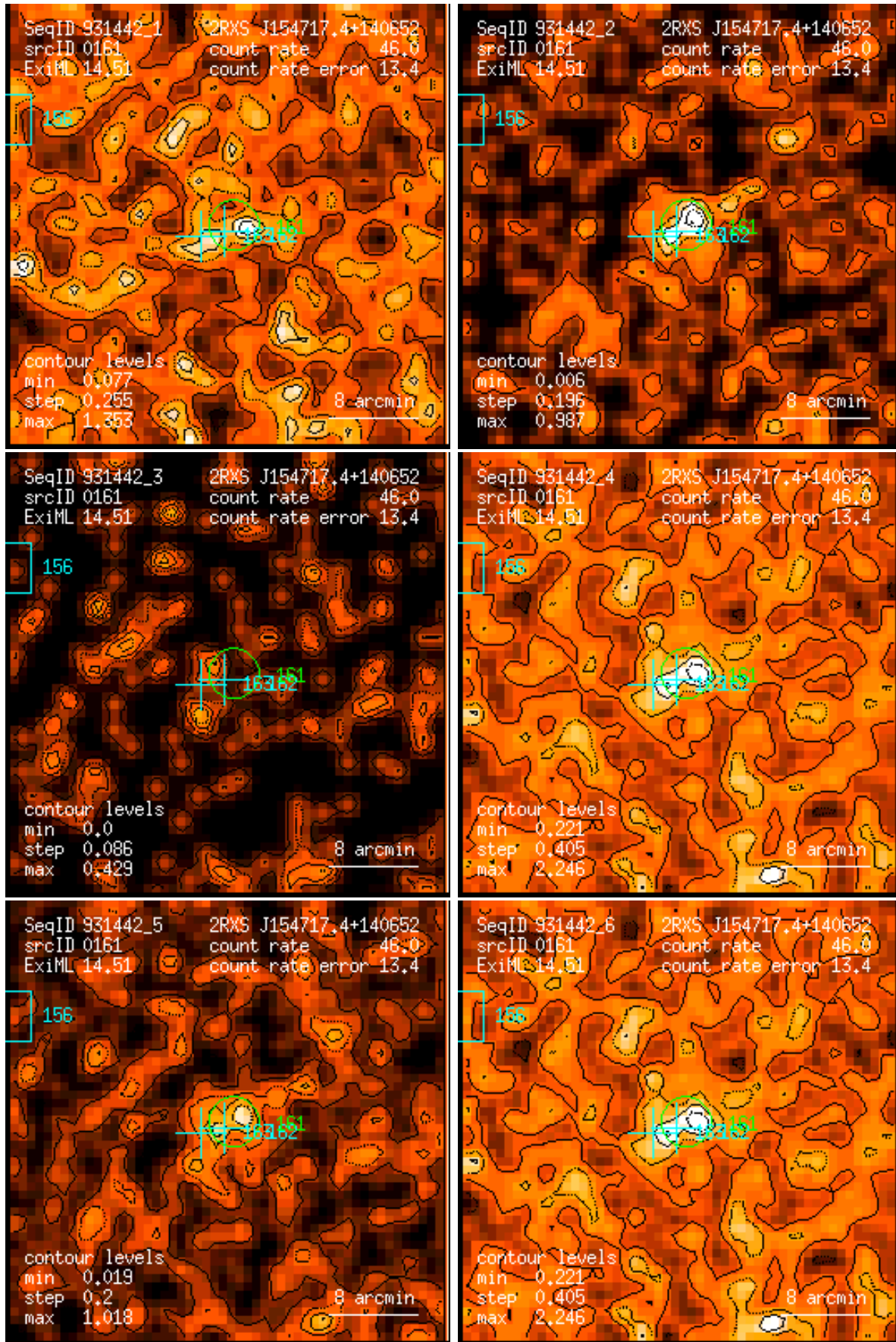
Figure 161: RASS 931442: detection 0161: band rate images, Gaussian filter: (1) PSPC channels 11 – 41, (2) 52 – 90, (3) 91 – 201, (4) 11 – 235, (5) 52 – 201, (6) 11 – 201. Broad band rates in counts/ks. Band rate contour levels in counts/ks/arcmin 2 .
