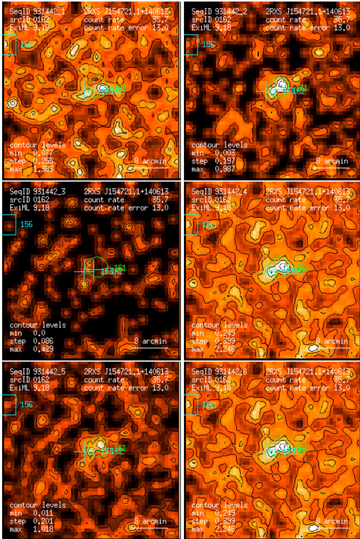
Figure 162: RASS 931442: detection 0162: band rate images, Gaussian filter: (1) PSPC channels 11 – 41, (2) 52 – 90, (3) 91 – 201, (4) 11 – 235, (5) 52 – 201, (6) 11 – 201. Broad band rates in counts/ks. Band rate contour levels in counts/ks/arcmin 2 .
