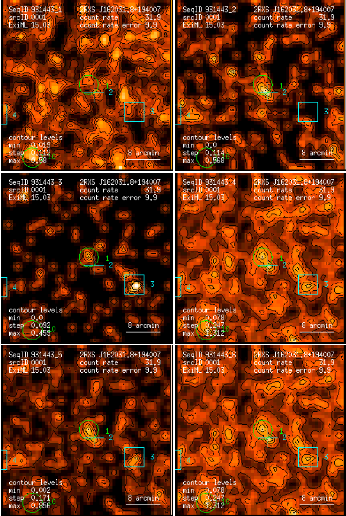
Figure 1: RASS 931443: detection 0001: band rate images, Gaussian filter: (1) PSPC channels 11 – 41, (2) 52 – 90, (3) 91 – 201, (4) 11 – 235, (5) 52 – 201, (6) 11 – 201. Broad band rates in counts/ks. Band rate contour levels in counts/ks/arcmin 2 .
