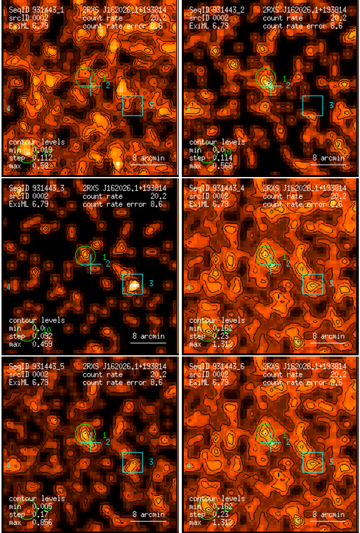
Figure 2: RASS 931443: detection 0002: band rate images, Gaussian filter: (1) PSPC channels 11 – 41, (2) 52 – 90, (3) 91 – 201, (4) 11 – 235, (5) 52 – 201, (6) 11 – 201. Broad band rates in counts/ks. Band rate contour levels in counts/ks/arcmin 2 .
