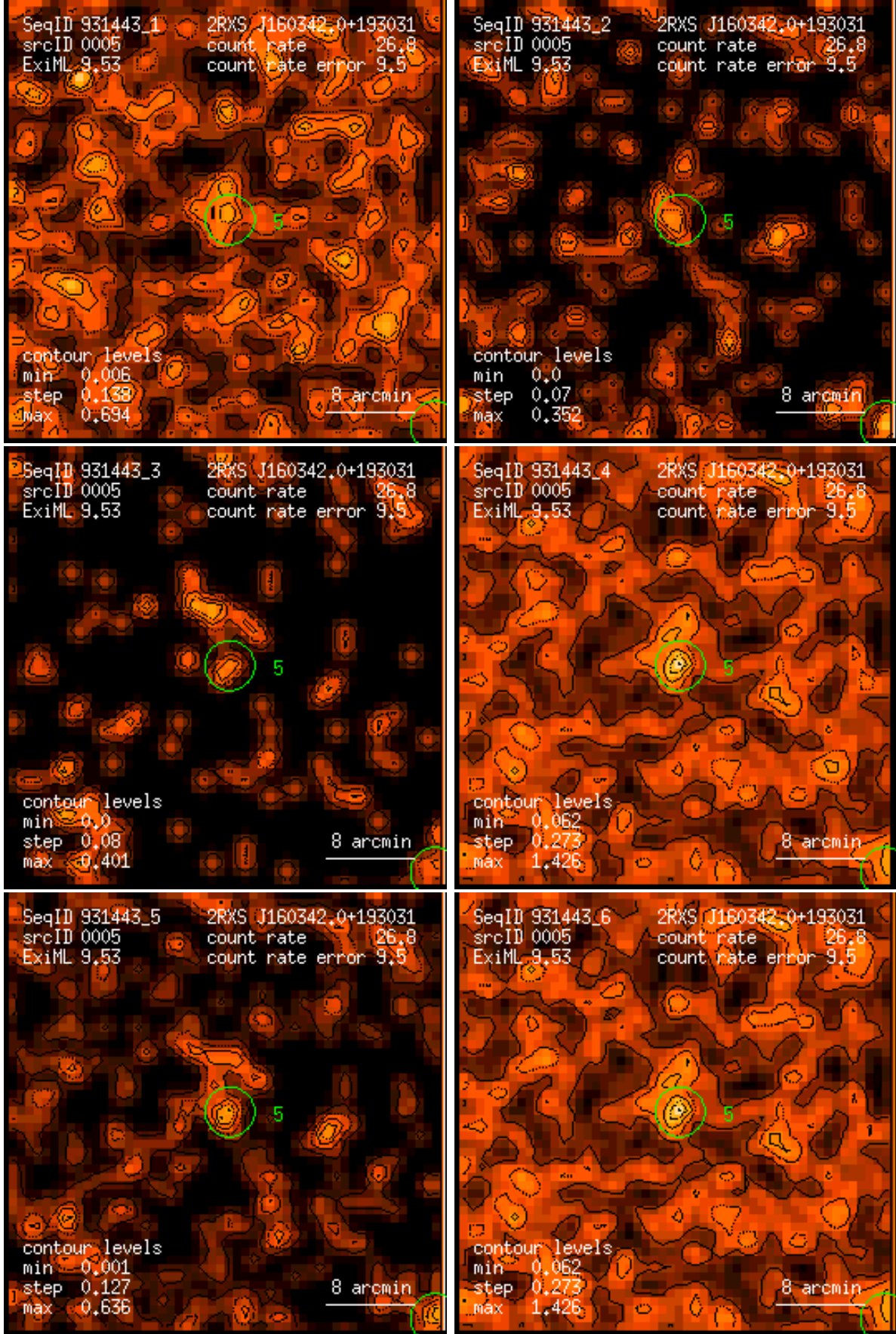
Figure 5: RASS 931443: detection 0005: band rate images, Gaussian filter: (1) PSPC channels 11 – 41, (2) 52 – 90, (3) 91 – 201, (4) 11 – 235, (5) 52 – 201, (6) 11 – 201. Broad band rates in counts/ks. Band rate contour levels in counts/ks/arcmin 2 .
