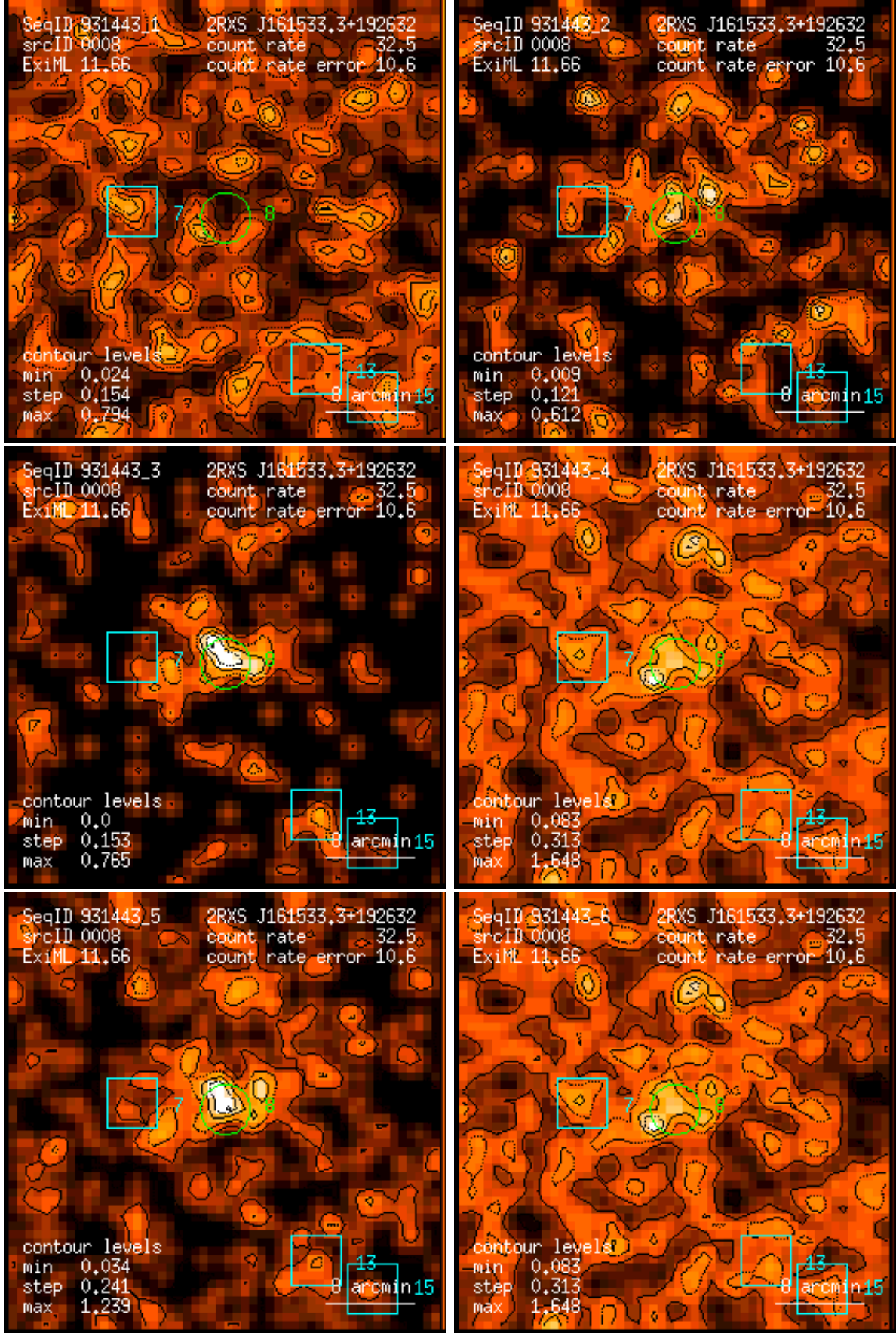
Figure 8: RASS 931443: detection 0008: band rate images, Gaussian filter: (1) PSPC channels 11 – 41, (2) 52 – 90, (3) 91 – 201, (4) 11 – 235, (5) 52 – 201, (6) 11 – 201. Broad band rates in counts/ks. Band rate contour levels in counts/ks/arcmin 2 .
