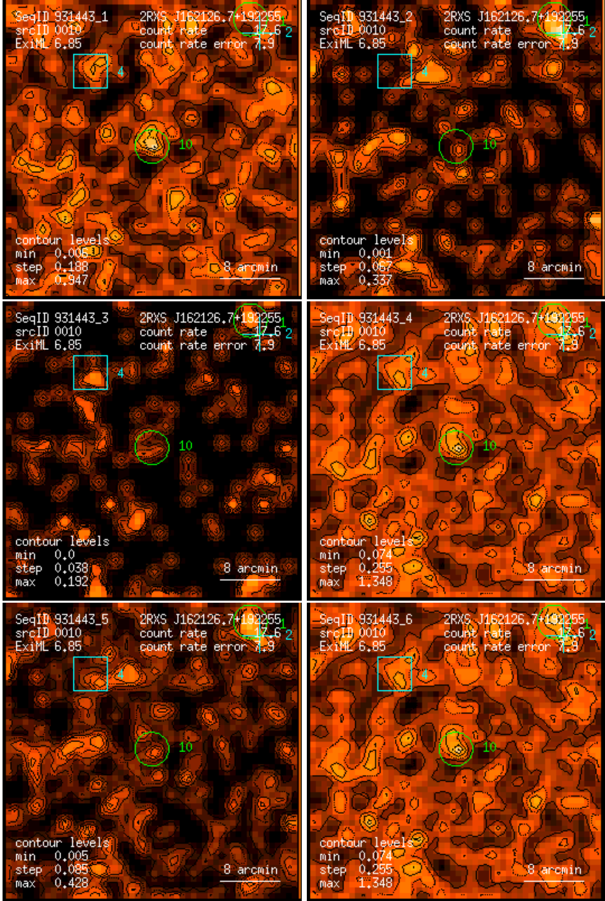
Figure 10: RASS 931443: detection 0010: band rate images, Gaussian filter: (1) PSPC channels 11 – 41, (2) 52 – 90, (3) 91 – 201, (4) 11 – 235, (5) 52 – 201, (6) 11 – 201. Broad band rates in counts/ks. Band rate contour levels in counts/ks/arcmin 2 .
