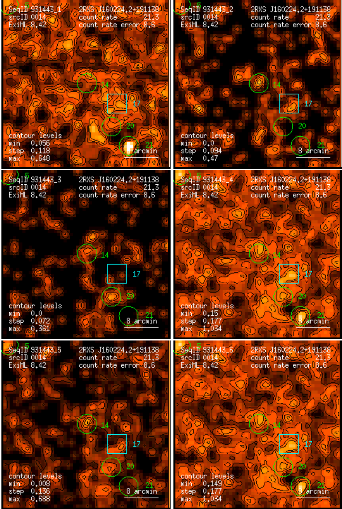
Figure 14: RASS 931443: detection 0014: band rate images, Gaussian filter: (1) PSPC channels 11 – 41, (2) 52 – 90, (3) 91 – 201, (4) 11 – 235, (5) 52 – 201, (6) 11 – 201. Broad band rates in counts/ks. Band rate contour levels in counts/ks/arcmin 2 .
