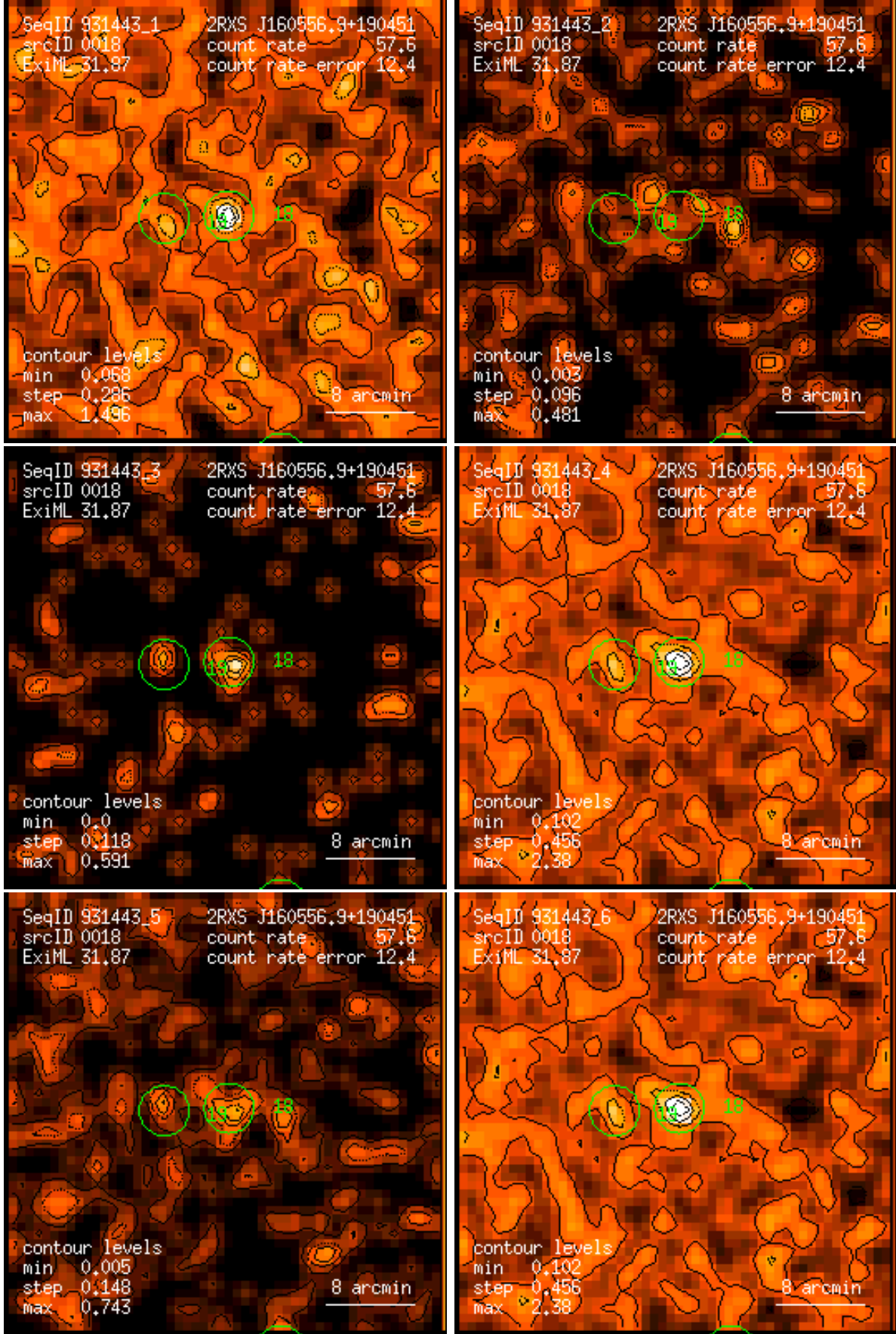
Figure 18: RASS 931443: detection 0018: band rate images, Gaussian filter: (1) PSPC channels 11 – 41, (2) 52 – 90, (3) 91 – 201, (4) 11 – 235, (5) 52 – 201, (6) 11 – 201. Broad band rates in counts/ks. Band rate contour levels in counts/ks/arcmin 2 .
