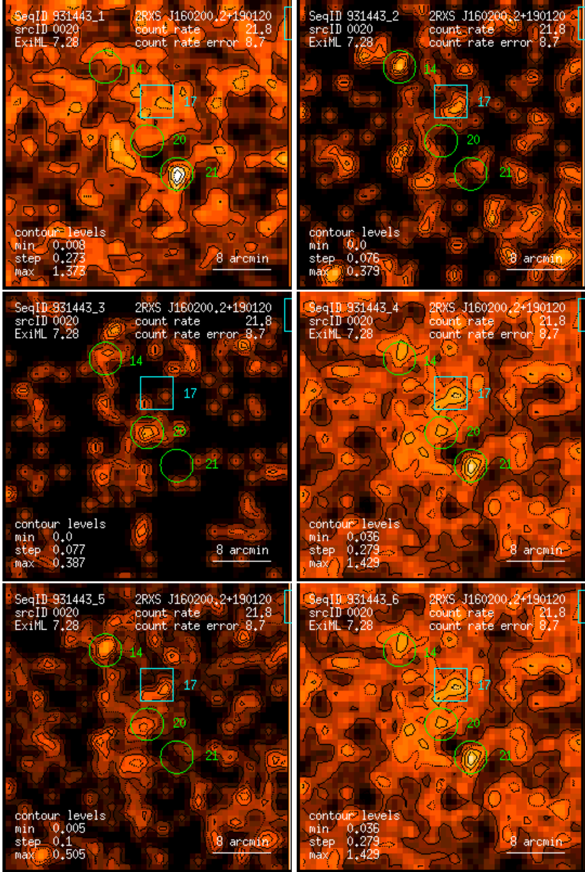
Figure 20: RASS 931443: detection 0020: band rate images, Gaussian filter: (1) PSPC channels 11 – 41, (2) 52 – 90, (3) 91 – 201, (4) 11 – 235, (5) 52 – 201, (6) 11 – 201. Broad band rates in counts/ks. Band rate contour levels in counts/ks/arcmin 2 .
