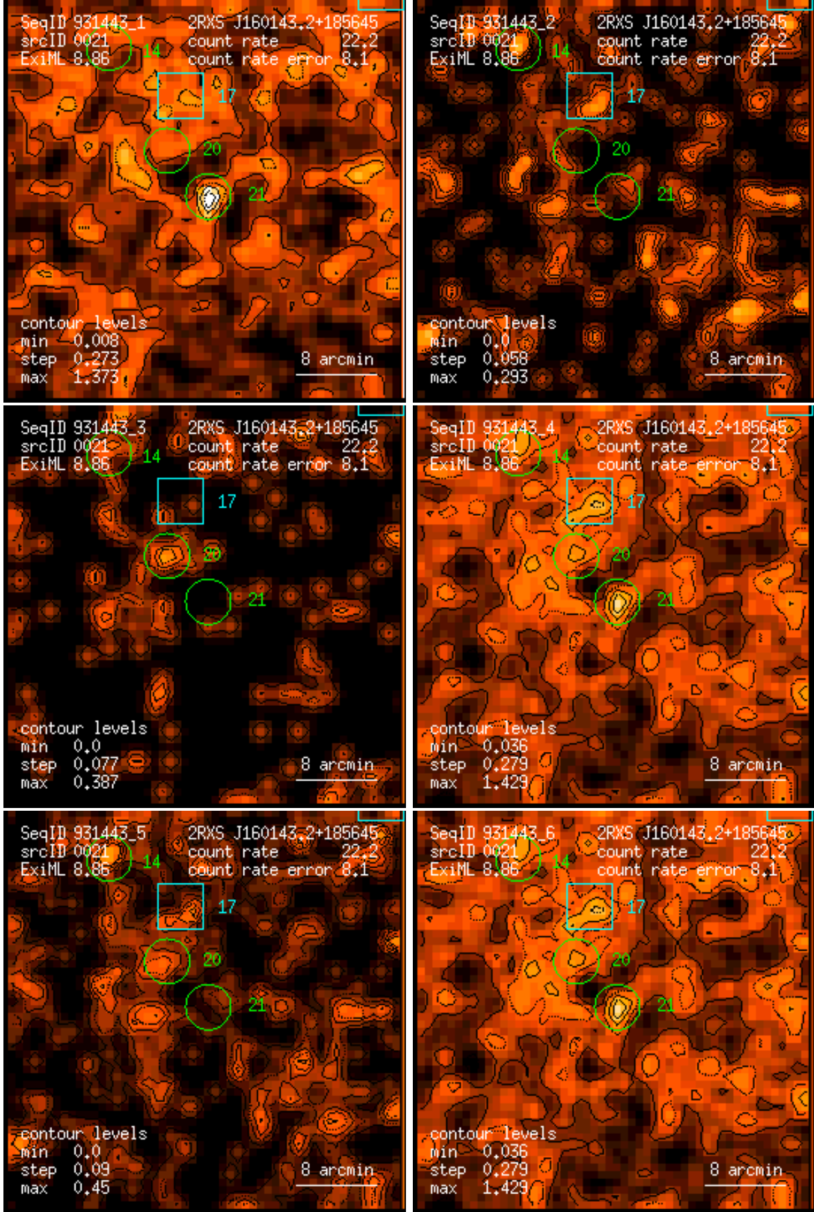
Figure 21: RASS 931443: detection 0021: band rate images, Gaussian filter: (1) PSPC channels 11 – 41, (2) 52 – 90, (3) 91 – 201, (4) 11 – 235, (5) 52 – 201, (6) 11 – 201. Broad band rates in counts/ks. Band rate contour levels in counts/ks/arcmin 2 .
