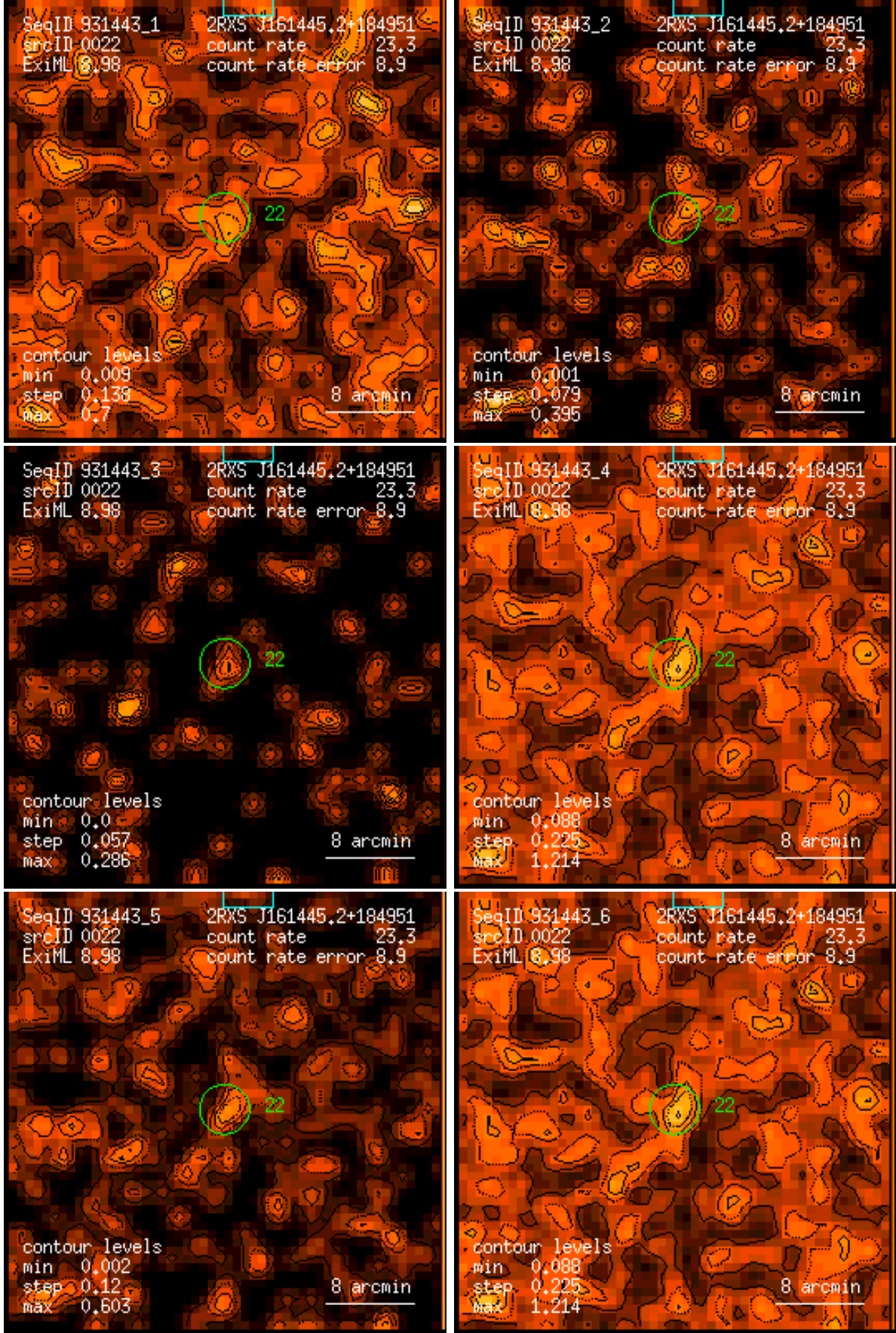
Figure 22: RASS 931443: detection 0022: band rate images, Gaussian filter: (1) PSPC channels 11 – 41, (2) 52 – 90, (3) 91 – 201, (4) 11 – 235, (5) 52 – 201, (6) 11 – 201. Broad band rates in counts/ks. Band rate contour levels in counts/ks/arcmin 2 .
