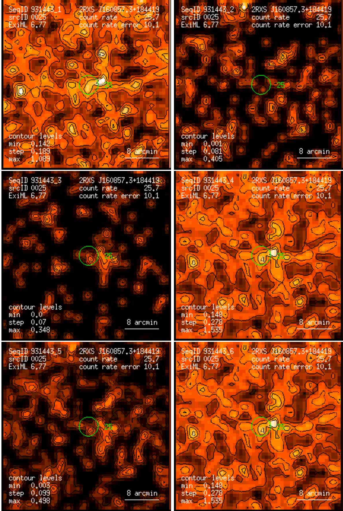
Figure 25: RASS 931443: detection 0025: band rate images, Gaussian filter: (1) PSPC channels 11 – 41, (2) 52 – 90, (3) 91 – 201, (4) 11 – 235, (5) 52 – 201, (6) 11 – 201. Broad band rates in counts/ks. Band rate contour levels in counts/ks/arcmin 2 .
