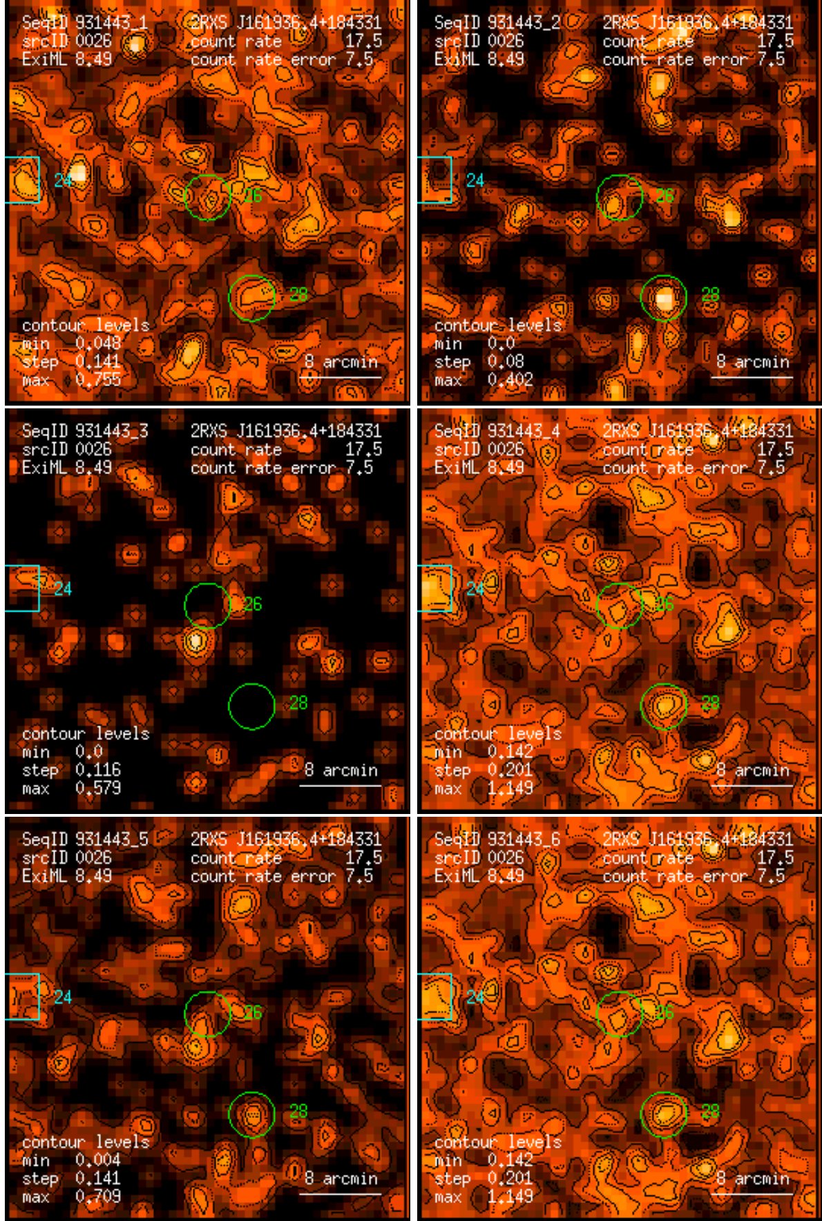
Figure 26: RASS 931443: detection 0026: band rate images, Gaussian filter: (1) PSPC channels 11 – 41, (2) 52 – 90, (3) 91 – 201, (4) 11 – 235, (5) 52 – 201, (6) 11 – 201. Broad band rates in counts/ks. Band rate contour levels in counts/ks/arcmin 2 .
