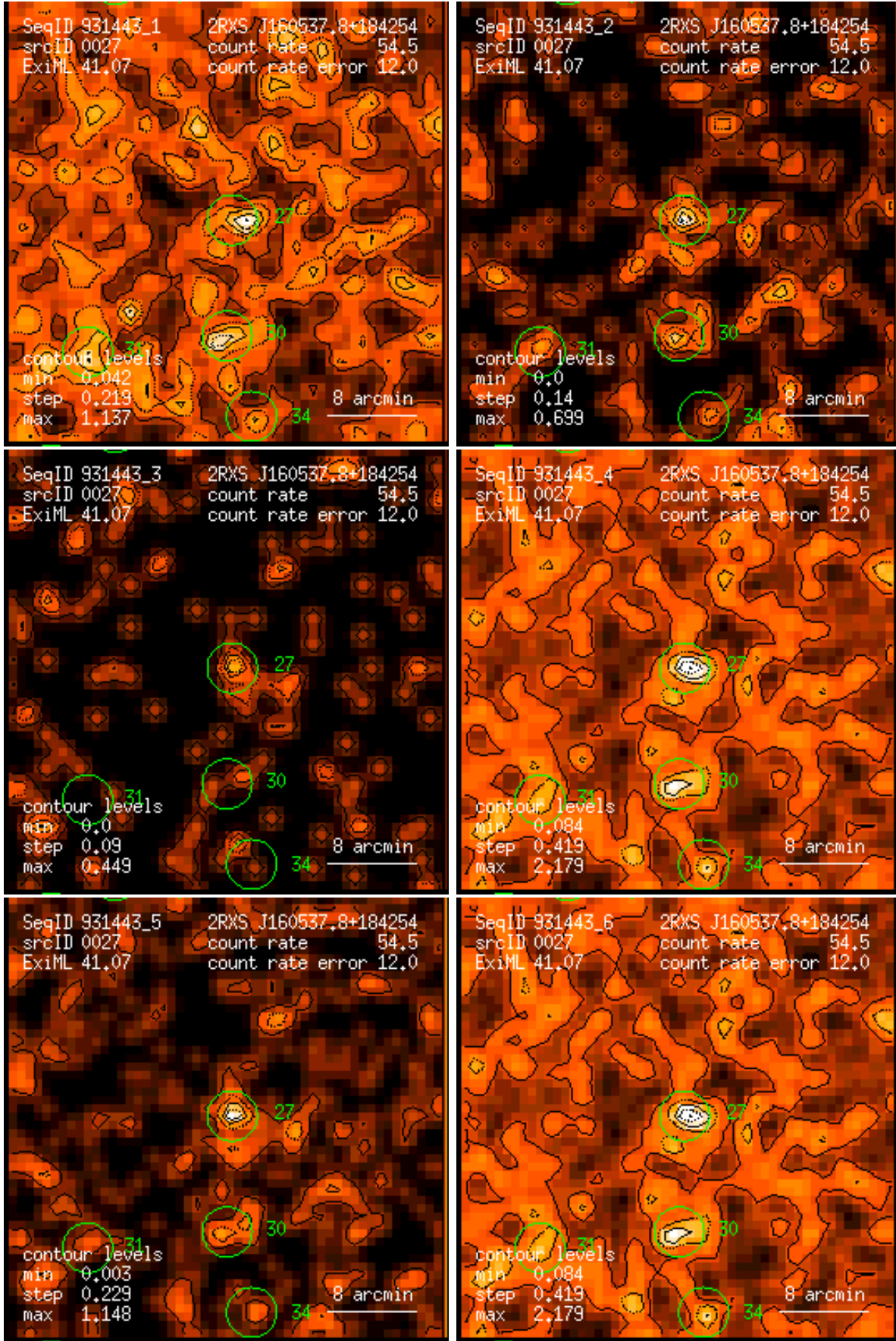
Figure 27: RASS 931443: detection 0027: band rate images, Gaussian filter: (1) PSPC channels 11 – 41, (2) 52 – 90, (3) 91 – 201, (4) 11 – 235, (5) 52 – 201, (6) 11 – 201. Broad band rates in counts/ks. Band rate contour levels in counts/ks/arcmin 2 .
