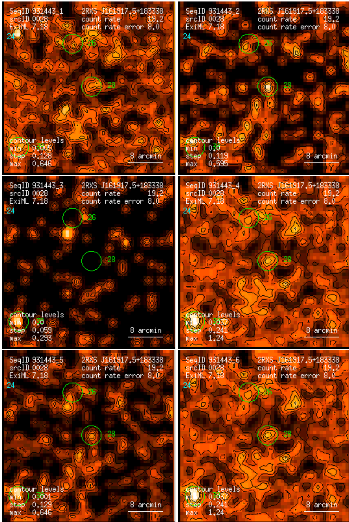
Figure 28: RASS 931443: detection 0028: band rate images, Gaussian filter: (1) PSPC channels 11 – 41, (2) 52 – 90, (3) 91 – 201, (4) 11 – 235, (5) 52 – 201, (6) 11 – 201. Broad band rates in counts/ks. Band rate contour levels in counts/ks/arcmin 2 .
