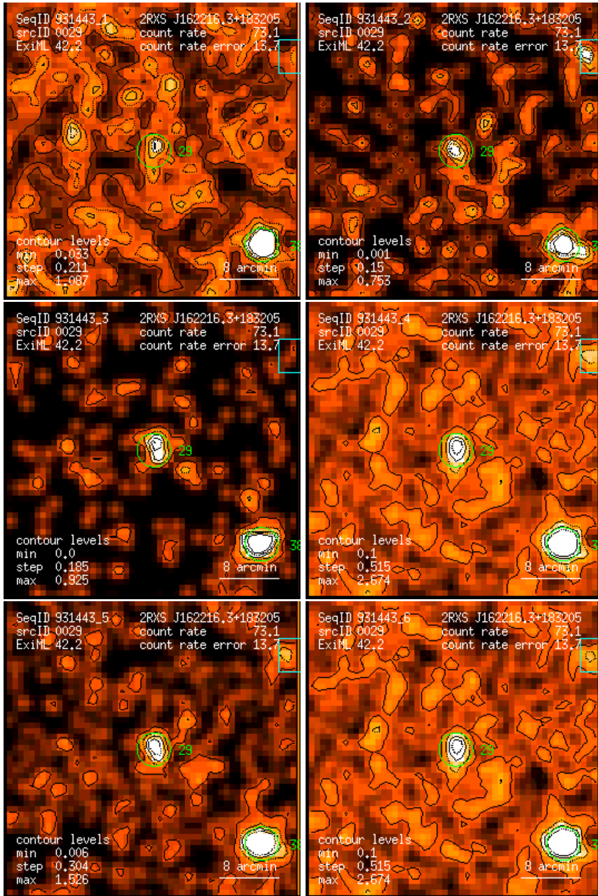
Figure 29: RASS 931443: detection 0029: band rate images, Gaussian filter: (1) PSPC channels 11 – 41, (2) 52 – 90, (3) 91 – 201, (4) 11 – 235, (5) 52 – 201, (6) 11 – 201. Broad band rates in counts/ks. Band rate contour levels in counts/ks/arcmin 2 .
