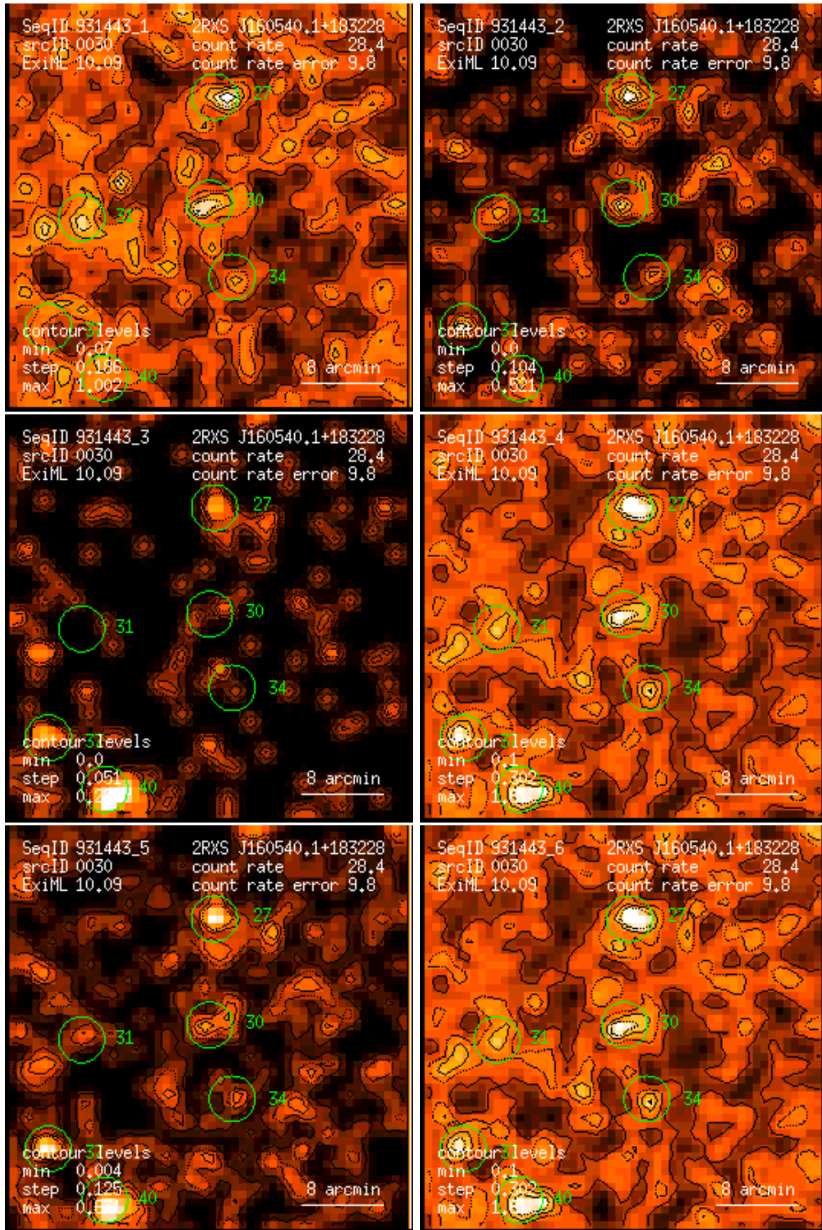
Figure 30: RASS 931443: detection 0030: band rate images, Gaussian filter: (1) PSPC channels 11 – 41, (2) 52 – 90, (3) 91 – 201, (4) 11 – 235, (5) 52 – 201, (6) 11 – 201. Broad band rates in counts/ks. Band rate contour levels in counts/ks/arcmin 2 .
