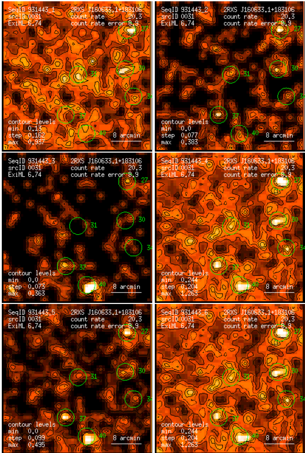
Figure 31: RASS 931443: detection 0031: band rate images, Gaussian filter: (1) PSPC channels 11 – 41, (2) 52 – 90, (3) 91 – 201, (4) 11 – 235, (5) 52 – 201, (6) 11 – 201. Broad band rates in counts/ks. Band rate contour levels in counts/ks/arcmin 2 .
