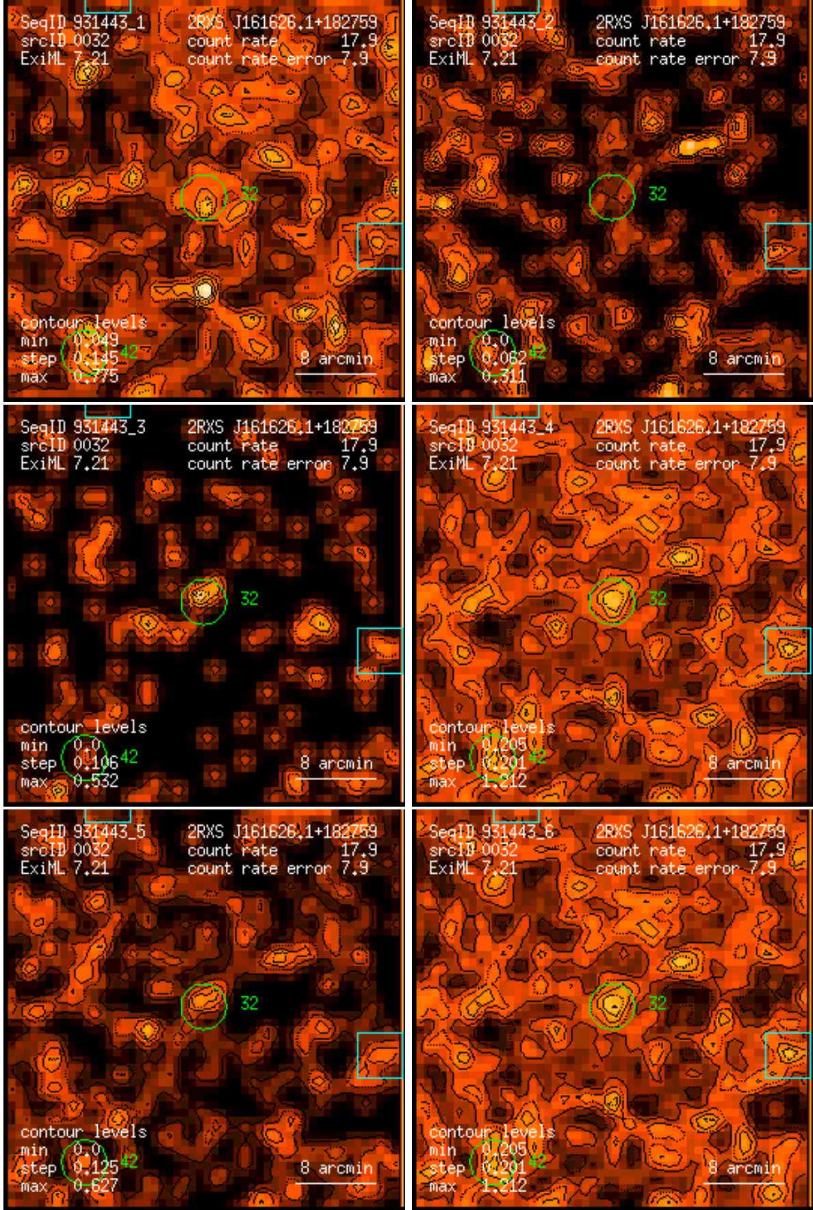
Figure 32: RASS 931443: detection 0032: band rate images, Gaussian filter: (1) PSPC channels 11 – 41, (2) 52 – 90, (3) 91 – 201, (4) 11 – 235, (5) 52 – 201, (6) 11 – 201. Broad band rates in counts/ks. Band rate contour levels in counts/ks/arcmin 2 .
