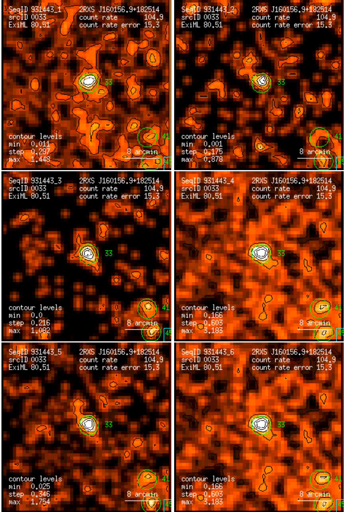
Figure 33: RASS 931443: detection 0033: band rate images, Gaussian filter: (1) PSPC channels 11 – 41, (2) 52 – 90, (3) 91 – 201, (4) 11 – 235, (5) 52 – 201, (6) 11 – 201. Broad band rates in counts/ks. Band rate contour levels in counts/ks/arcmin 2 .
