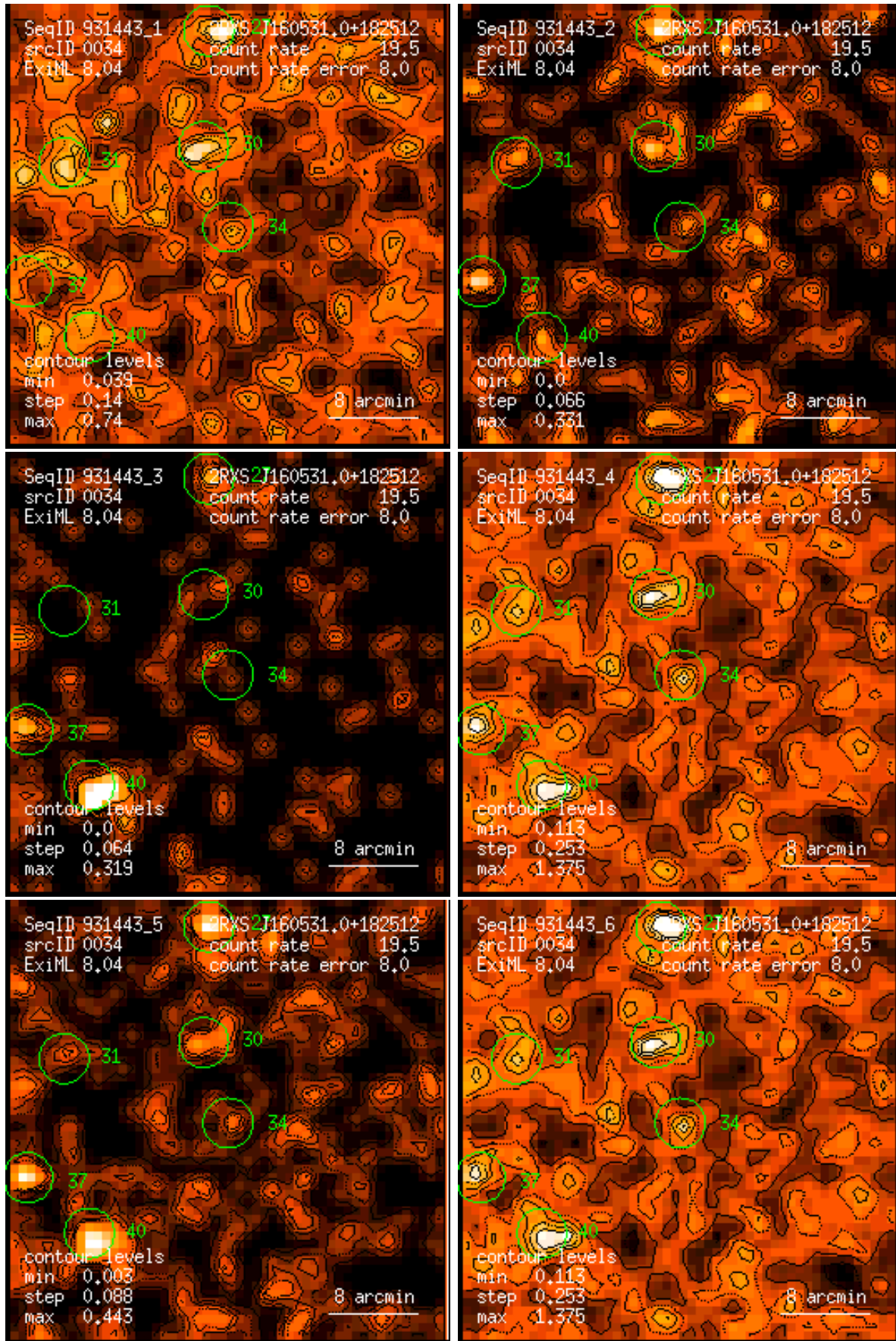
Figure 34: RASS 931443: detection 0034: band rate images, Gaussian filter: (1) PSPC channels 11 – 41, (2) 52 – 90, (3) 91 – 201, (4) 11 – 235, (5) 52 – 201, (6) 11 – 201. Broad band rates in counts/ks. Band rate contour levels in counts/ks/arcmin 2 .
