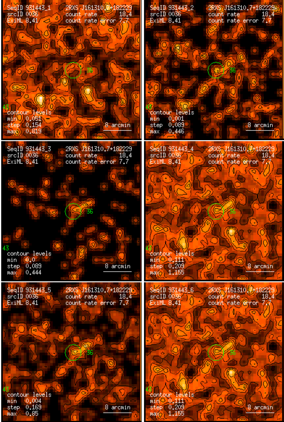
Figure 36: RASS 931443: detection 0036: band rate images, Gaussian filter: (1) PSPC channels 11 – 41, (2) 52 – 90, (3) 91 – 201, (4) 11 – 235, (5) 52 – 201, (6) 11 – 201. Broad band rates in counts/ks. Band rate contour levels in counts/ks/arcmin 2 .
