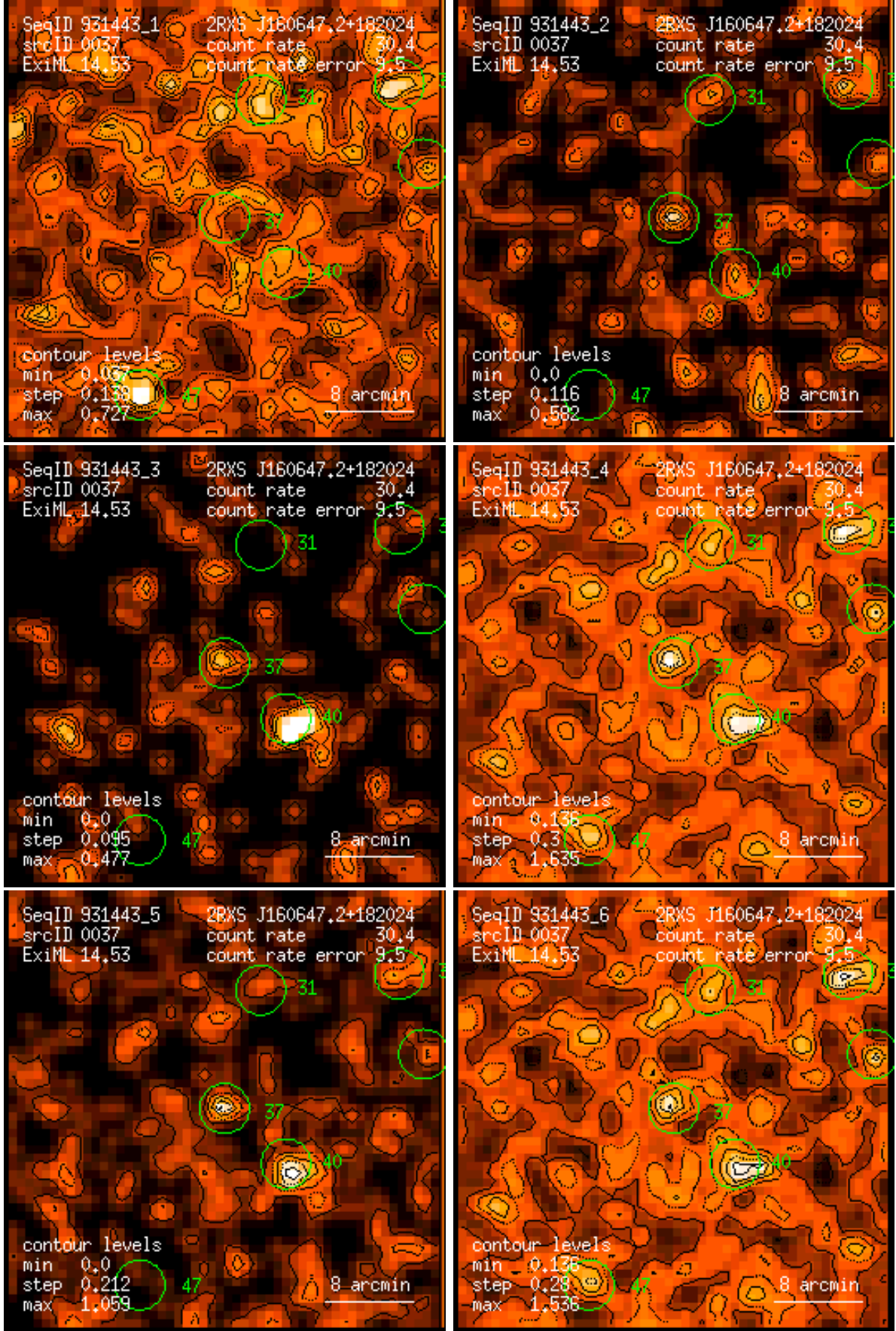
Figure 37: RASS 931443: detection 0037: band rate images, Gaussian filter: (1) PSPC channels 11 – 41, (2) 52 – 90, (3) 91 – 201, (4) 11 – 235, (5) 52 – 201, (6) 11 – 201. Broad band rates in counts/ks. Band rate contour levels in counts/ks/arcmin 2 .
