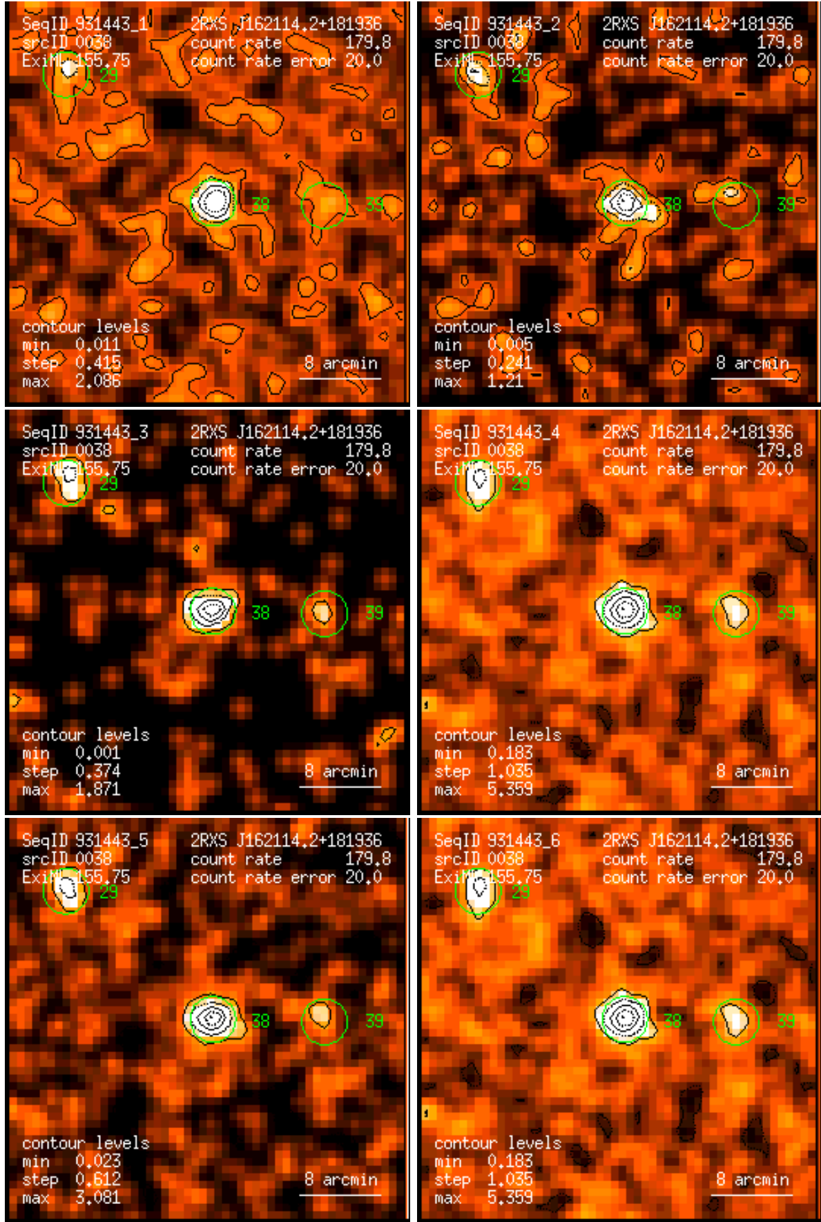
Figure 38: RASS 931443: detection 0038: band rate images, Gaussian filter: (1) PSPC channels 11 – 41, (2) 52 – 90, (3) 91 – 201, (4) 11 – 235, (5) 52 – 201, (6) 11 – 201. Broad band rates in counts/ks. Band rate contour levels in counts/ks/arcmin 2 .
