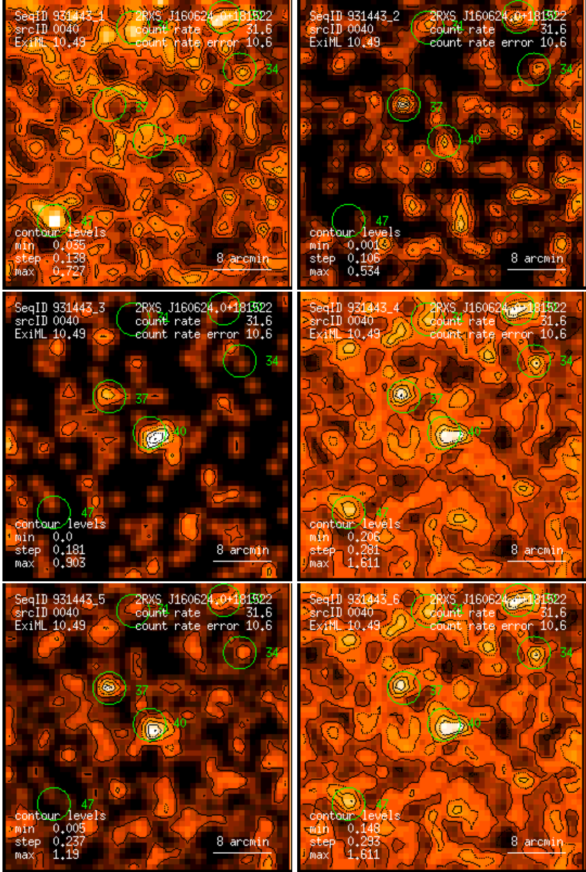
Figure 40: RASS 931443: detection 0040: band rate images, Gaussian filter: (1) PSPC channels 11 – 41, (2) 52 – 90, (3) 91 – 201, (4) 11 – 235, (5) 52 – 201, (6) 11 – 201. Broad band rates in counts/ks. Band rate contour levels in counts/ks/arcmin 2 .
