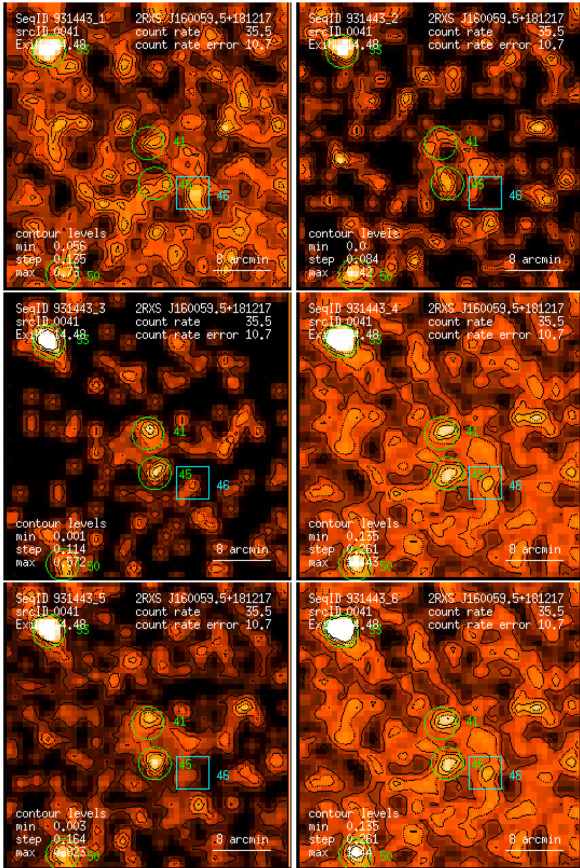
Figure 41: RASS 931443: detection 0041: band rate images, Gaussian filter: (1) PSPC channels 11 – 41, (2) 52 – 90, (3) 91 – 201, (4) 11 – 235, (5) 52 – 201, (6) 11 – 201. Broad band rates in counts/ks. Band rate contour levels in counts/ks/arcmin 2 .
