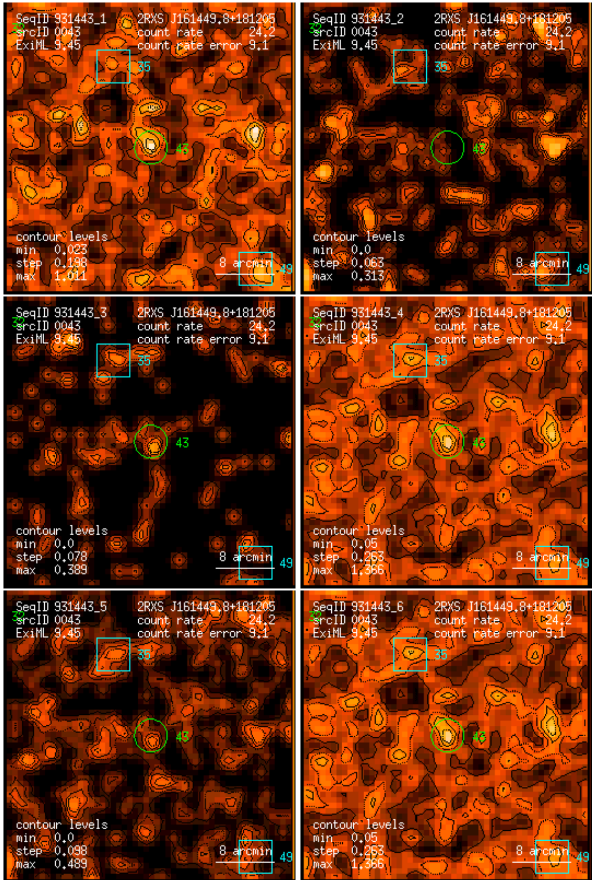
Figure 43: RASS 931443: detection 0043: band rate images, Gaussian filter: (1) PSPC channels 11 – 41, (2) 52 – 90, (3) 91 – 201, (4) 11 – 235, (5) 52 – 201, (6) 11 – 201. Broad band rates in counts/ks. Band rate contour levels in counts/ks/arcmin 2 .
