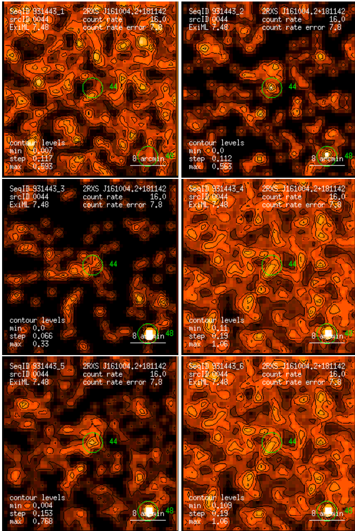
Figure 44: RASS 931443: detection 0044: band rate images, Gaussian filter: (1) PSPC channels 11 – 41, (2) 52 – 90, (3) 91 – 201, (4) 11 – 235, (5) 52 – 201, (6) 11 – 201. Broad band rates in counts/ks. Band rate contour levels in counts/ks/arcmin 2 .
