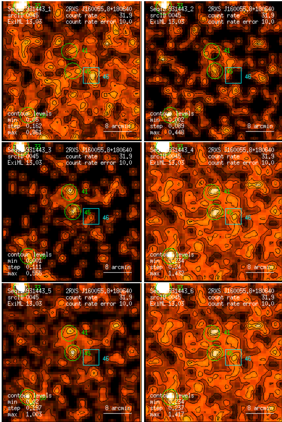
Figure 45: RASS 931443: detection 0045: band rate images, Gaussian filter: (1) PSPC channels 11 – 41, (2) 52 – 90, (3) 91 – 201, (4) 11 – 235, (5) 52 – 201, (6) 11 – 201. Broad band rates in counts/ks. Band rate contour levels in counts/ks/arcmin 2 .
