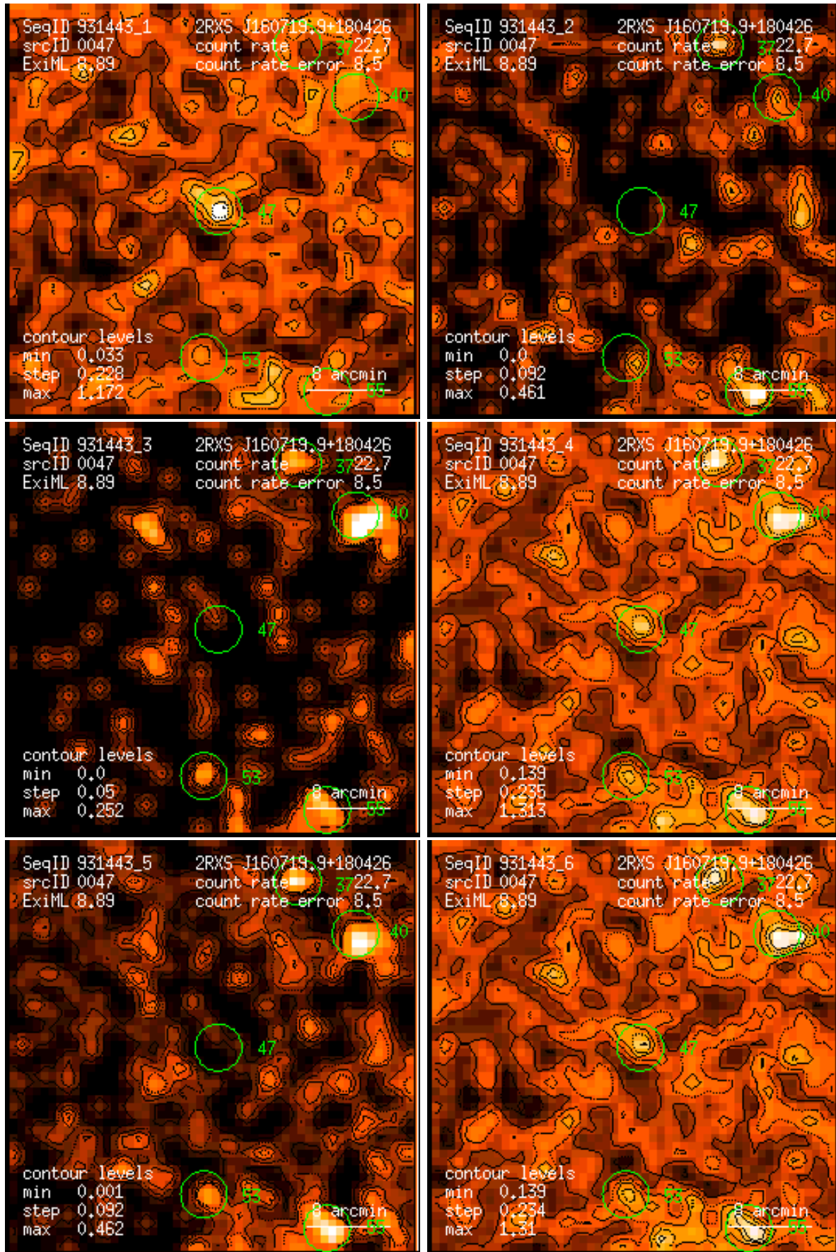
Figure 47: RASS 931443: detection 0047: band rate images, Gaussian filter: (1) PSPC channels 11 – 41, (2) 52 – 90, (3) 91 – 201, (4) 11 – 235, (5) 52 – 201, (6) 11 – 201. Broad band rates in counts/ks. Band rate contour levels in counts/ks/arcmin 2 .
