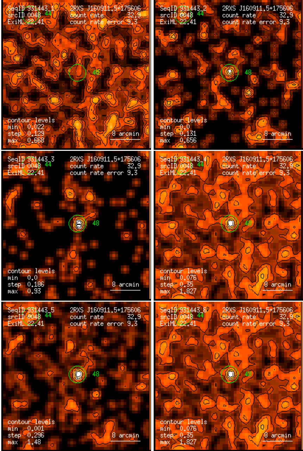
Figure 48: RASS 931443: detection 0048: band rate images, Gaussian filter: (1) PSPC channels 11 – 41, (2) 52 – 90, (3) 91 – 201, (4) 11 – 235, (5) 52 – 201, (6) 11 – 201. Broad band rates in counts/ks. Band rate contour levels in counts/ks/arcmin 2 .
