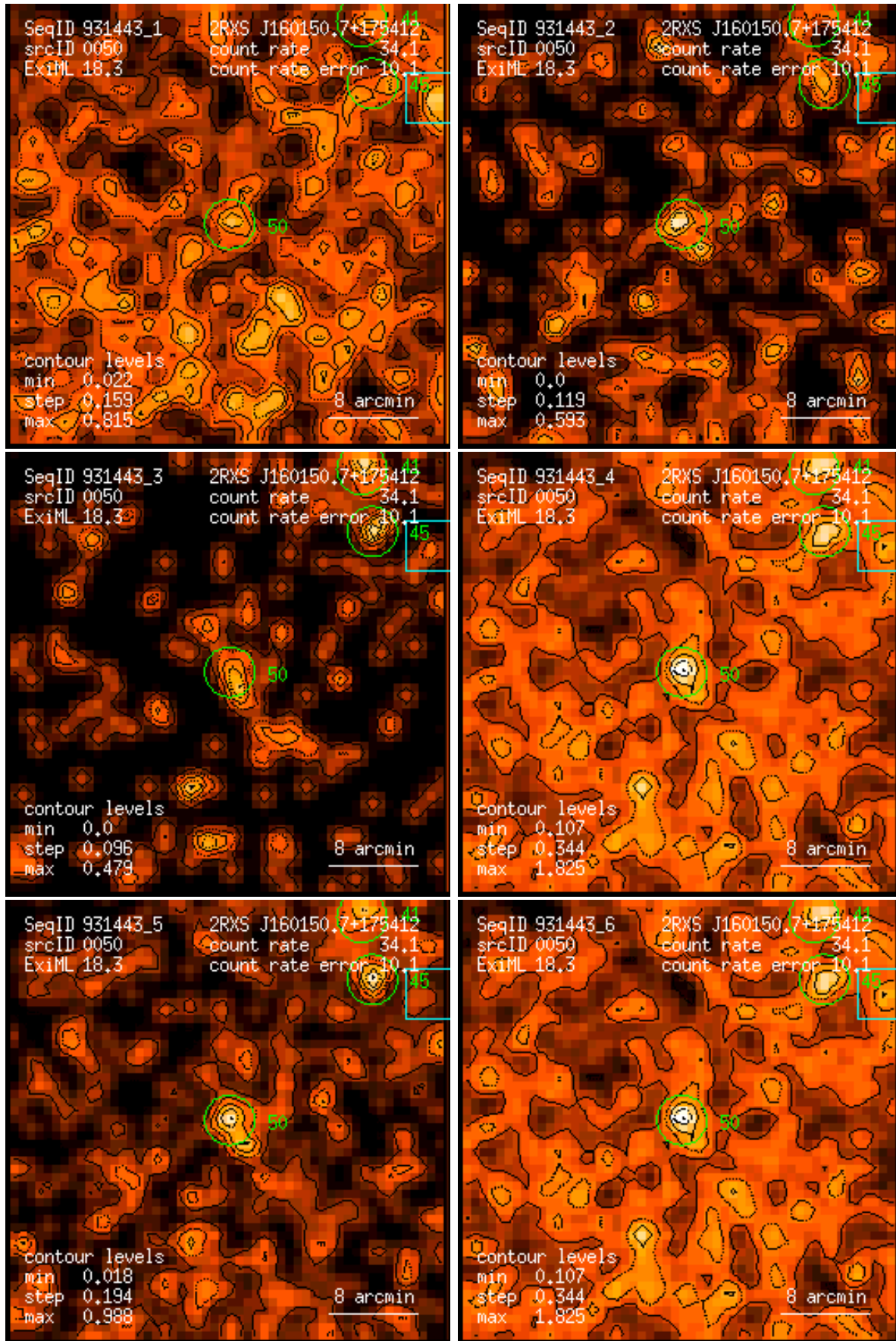
Figure 50: RASS 931443: detection 0050: band rate images, Gaussian filter: (1) PSPC channels 11 – 41, (2) 52 – 90, (3) 91 – 201, (4) 11 – 235, (5) 52 – 201, (6) 11 – 201. Broad band rates in counts/ks. Band rate contour levels in counts/ks/arcmin 2 .
