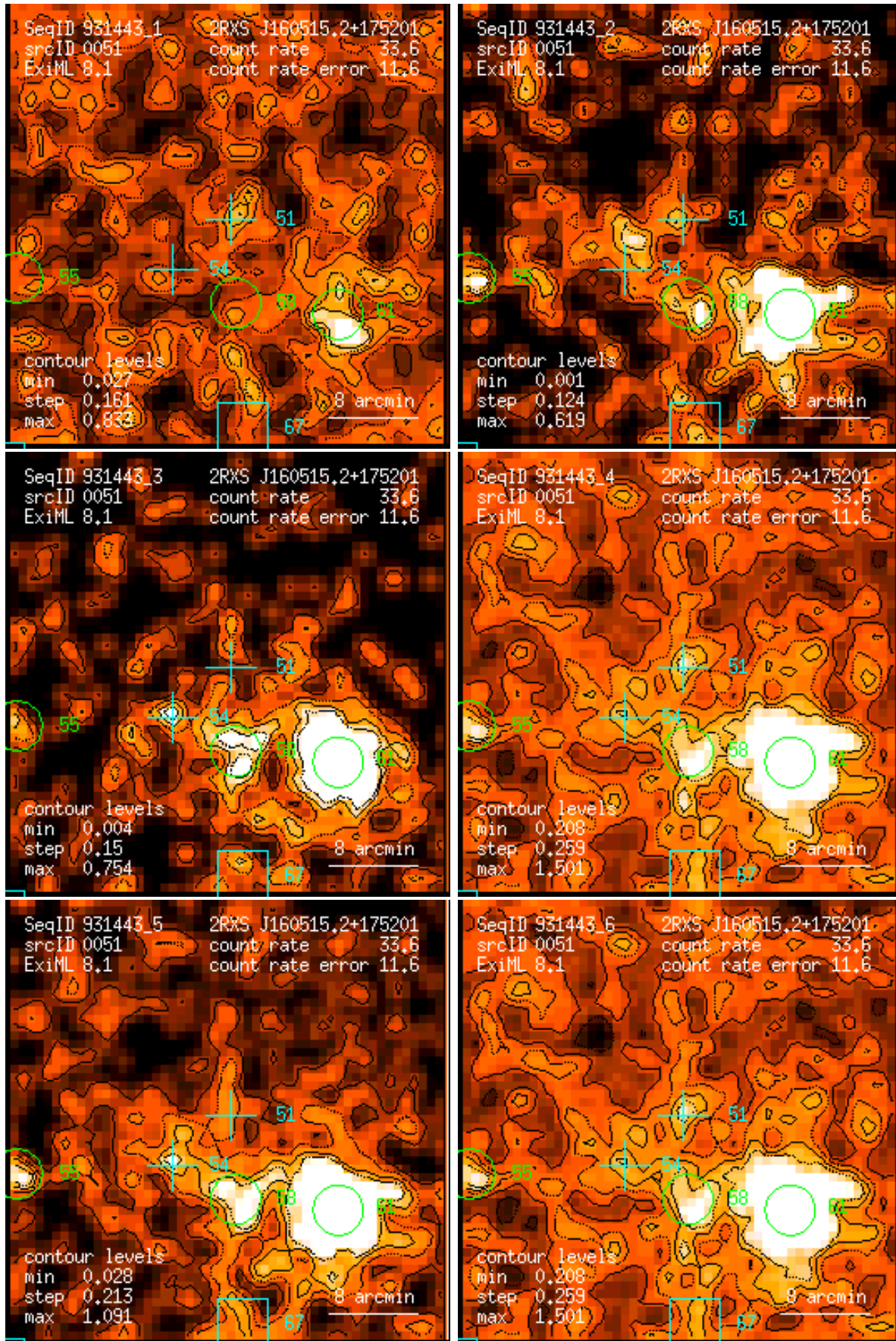
Figure 51: RASS 931443: detection 0051: band rate images, Gaussian filter: (1) PSPC channels 11 – 41, (2) 52 – 90, (3) 91 – 201, (4) 11 – 235, (5) 52 – 201, (6) 11 – 201. Broad band rates in counts/ks. Band rate contour levels in counts/ks/arcmin 2 .
