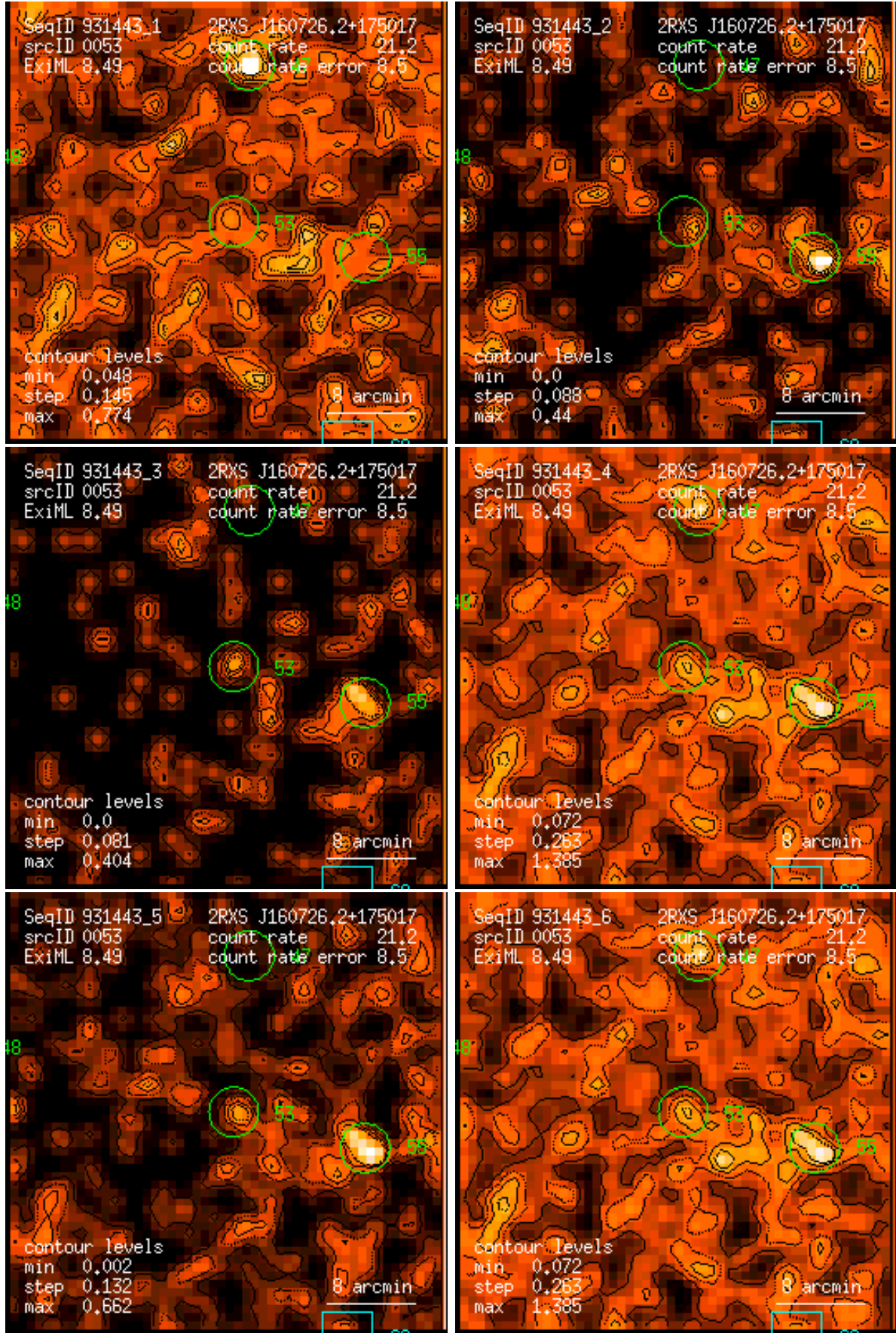
Figure 53: RASS 931443: detection 0053: band rate images, Gaussian filter: (1) PSPC channels 11 – 41, (2) 52 – 90, (3) 91 – 201, (4) 11 – 235, (5) 52 – 201, (6) 11 – 201. Broad band rates in counts/ks. Band rate contour levels in counts/ks/arcmin 2 .
