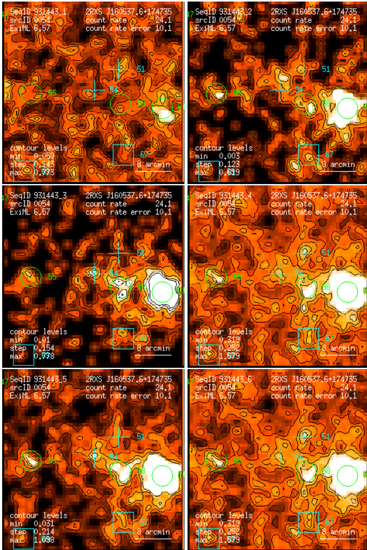
Figure 54: RASS 931443: detection 0054: band rate images, Gaussian filter: (1) PSPC channels 11 – 41, (2) 52 – 90, (3) 91 – 201, (4) 11 – 235, (5) 52 – 201, (6) 11 – 201. Broad band rates in counts/ks. Band rate contour levels in counts/ks/arcmin 2 .
