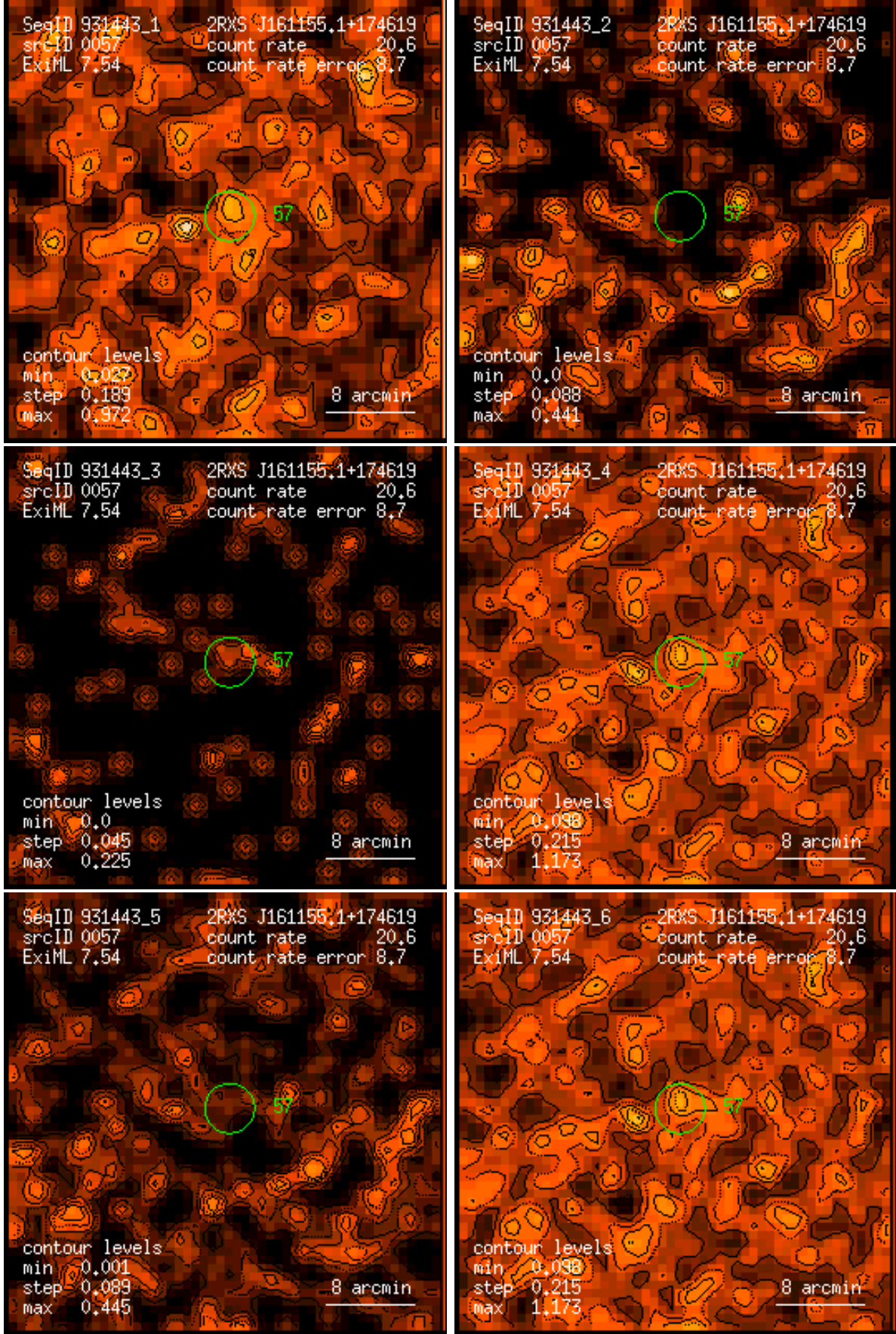
Figure 57: RASS 931443: detection 0057: band rate images, Gaussian filter: (1) PSPC channels 11 – 41, (2) 52 – 90, (3) 91 – 201, (4) 11 – 235, (5) 52 – 201, (6) 11 – 201. Broad band rates in counts/ks. Band rate contour levels in counts/ks/arcmin 2 .
