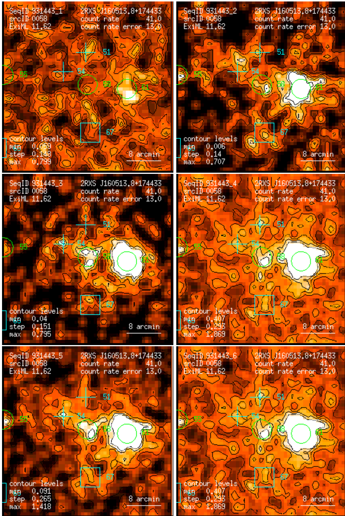
Figure 58: RASS 931443: detection 0058: band rate images, Gaussian filter: (1) PSPC channels 11 – 41, (2) 52 – 90, (3) 91 – 201, (4) 11 – 235, (5) 52 – 201, (6) 11 – 201. Broad band rates in counts/ks. Band rate contour levels in counts/ks/arcmin 2 .
