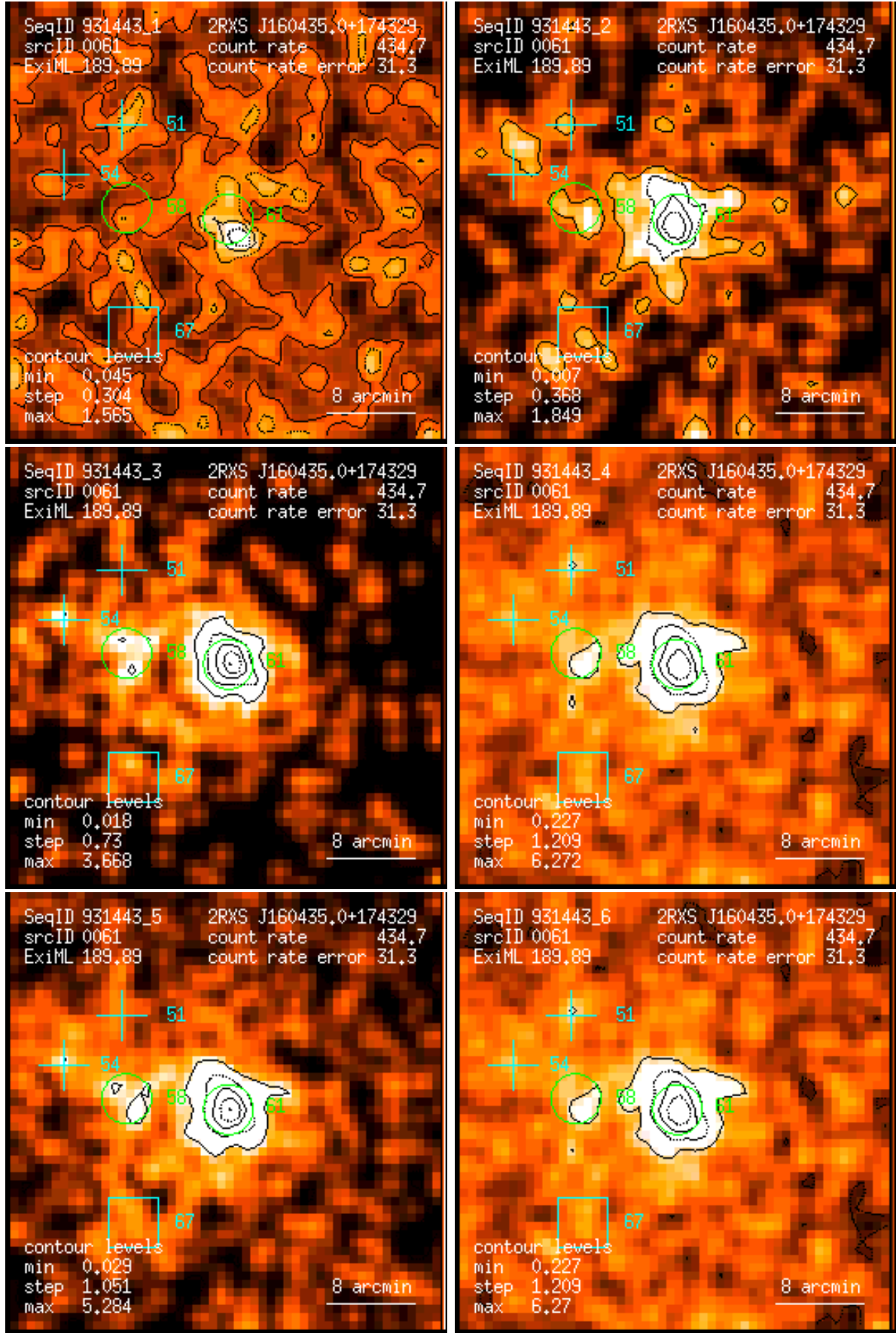
Figure 61: RASS 931443: detection 0061: band rate images, Gaussian filter: (1) PSPC channels 11 – 41, (2) 52 – 90, (3) 91 – 201, (4) 11 – 235, (5) 52 – 201, (6) 11 – 201. Broad band rates in counts/ks. Band rate contour levels in counts/ks/arcmin 2 .
