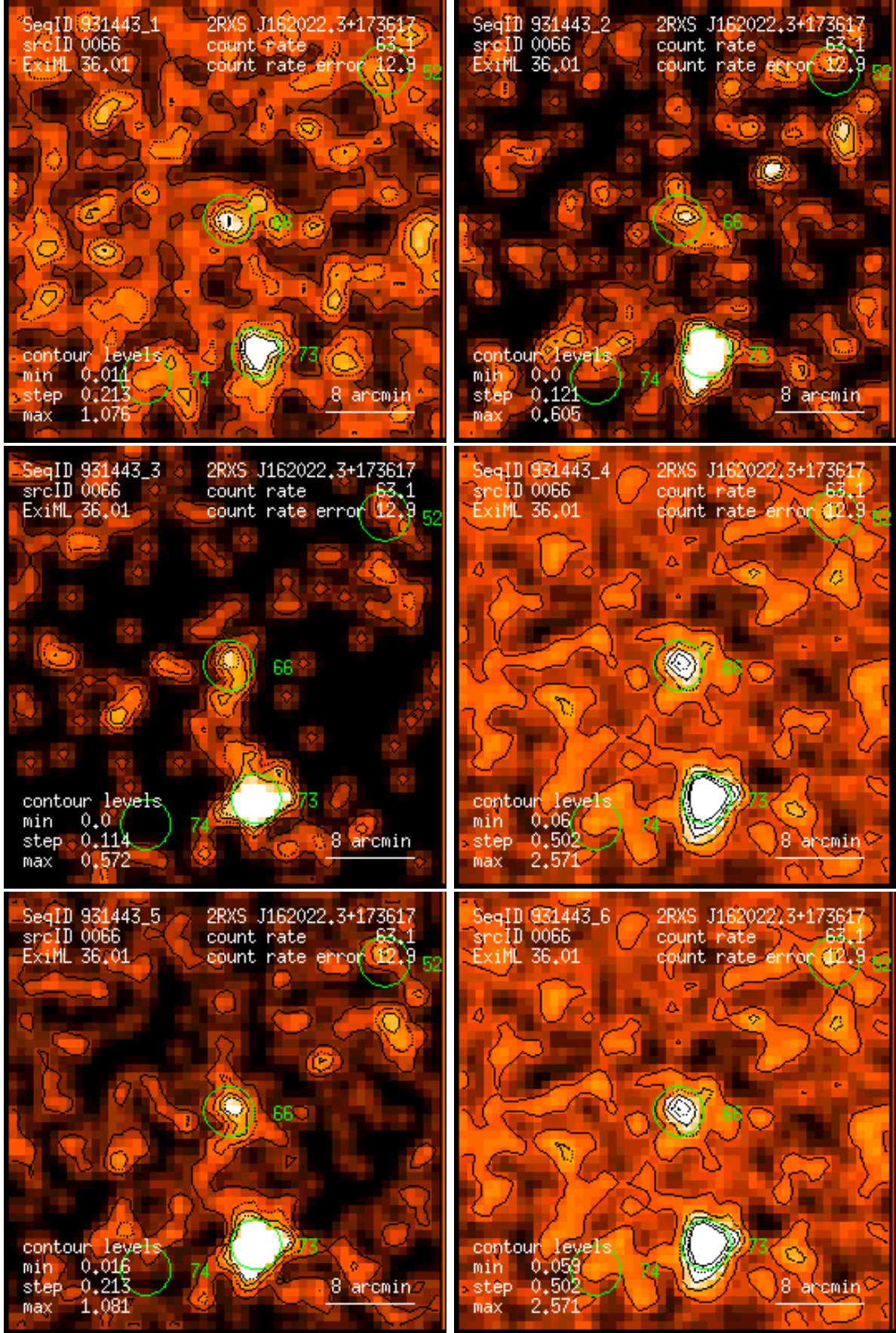
Figure 66: RASS 931443: detection 0066: band rate images, Gaussian filter: (1) PSPC channels 11 – 41, (2) 52 – 90, (3) 91 – 201, (4) 11 – 235, (5) 52 – 201, (6) 11 – 201. Broad band rates in counts/ks. Band rate contour levels in counts/ks/arcmin 2 .
