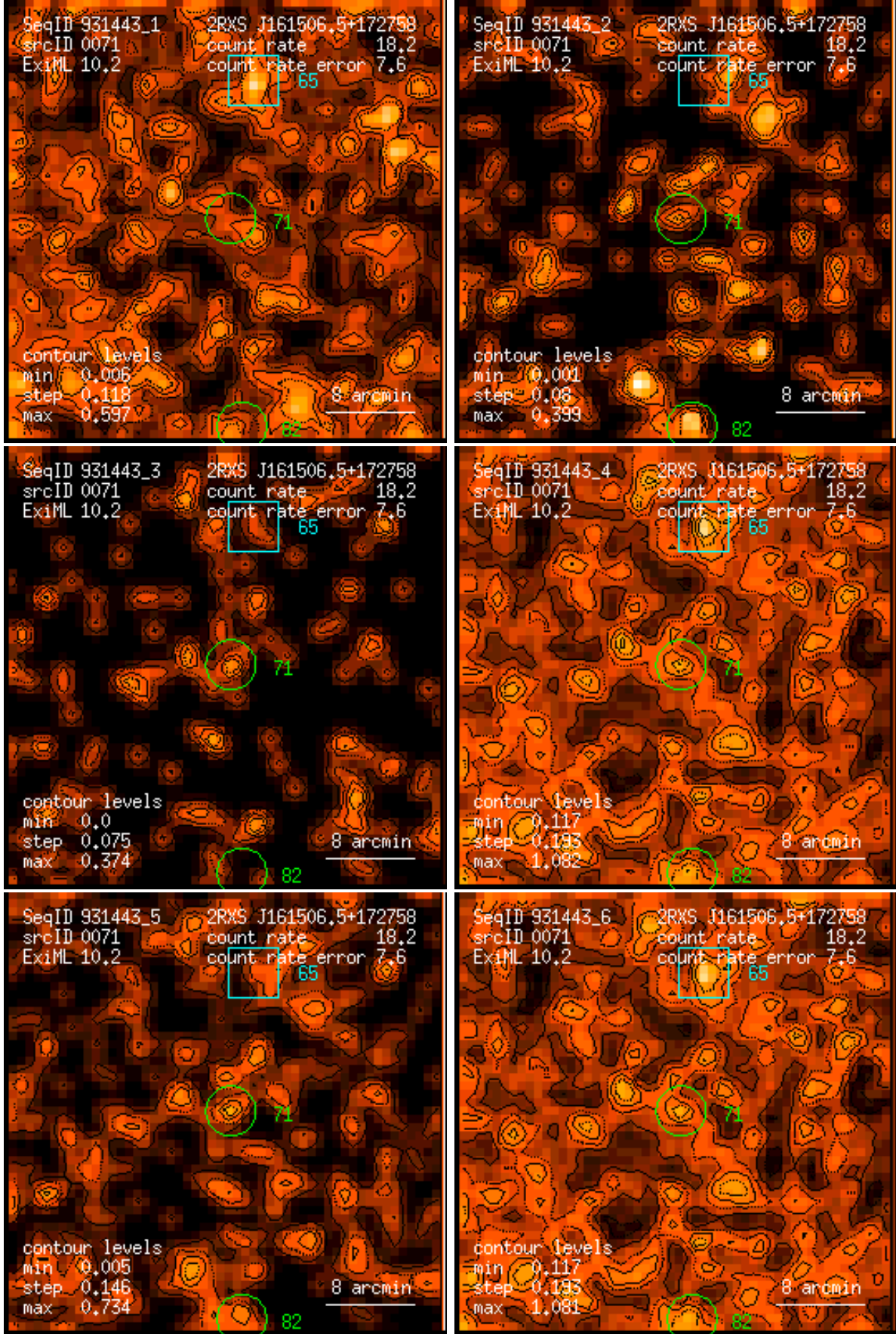
Figure 71: RASS 931443: detection 0071: band rate images, Gaussian filter: (1) PSPC channels 11 – 41, (2) 52 – 90, (3) 91 – 201, (4) 11 – 235, (5) 52 – 201, (6) 11 – 201. Broad band rates in counts/ks. Band rate contour levels in counts/ks/arcmin 2 .
