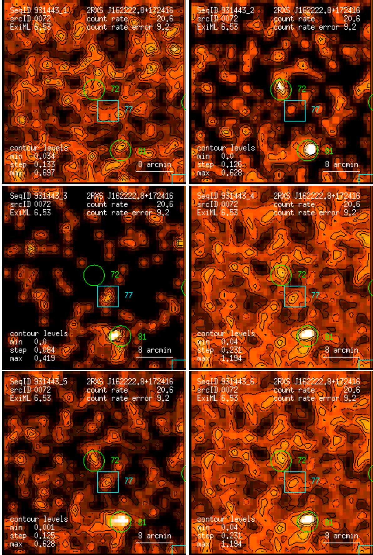
Figure 72: RASS 931443: detection 0072: band rate images, Gaussian filter: (1) PSPC channels 11 – 41, (2) 52 – 90, (3) 91 – 201, (4) 11 – 235, (5) 52 – 201, (6) 11 – 201. Broad band rates in counts/ks. Band rate contour levels in counts/ks/arcmin 2 .
