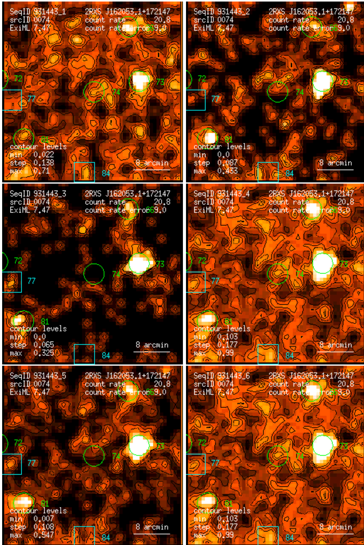
Figure 74: RASS 931443: detection 0074: band rate images, Gaussian filter: (1) PSPC channels 11 – 41, (2) 52 – 90, (3) 91 – 201, (4) 11 – 235, (5) 52 – 201, (6) 11 – 201. Broad band rates in counts/ks. Band rate contour levels in counts/ks/arcmin 2 .
