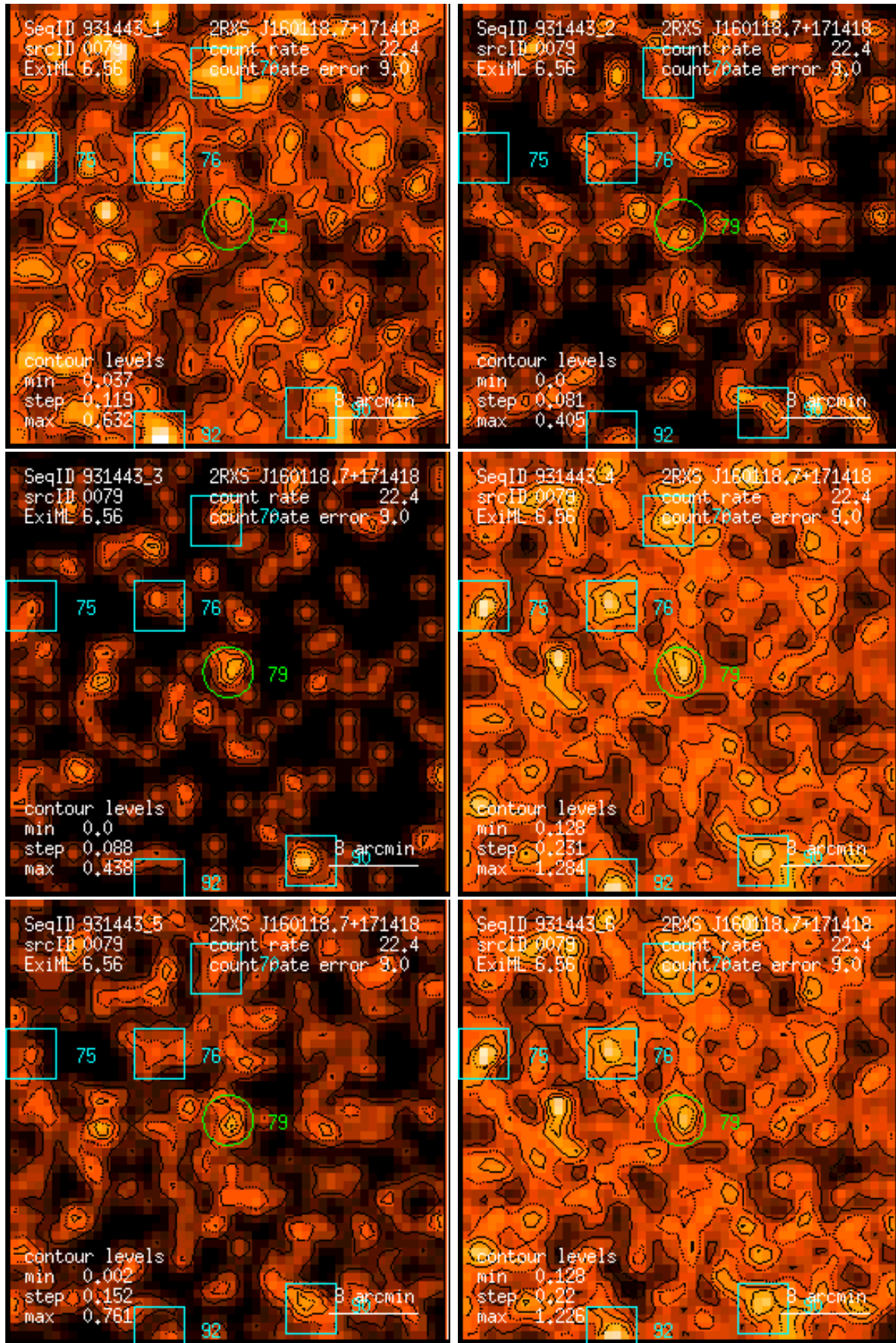
Figure 79: RASS 931443: detection 0079: band rate images, Gaussian filter: (1) PSPC channels 11 – 41, (2) 52 – 90, (3) 91 – 201, (4) 11 – 235, (5) 52 – 201, (6) 11 – 201. Broad band rates in counts/ks. Band rate contour levels in counts/ks/arcmin 2 .
