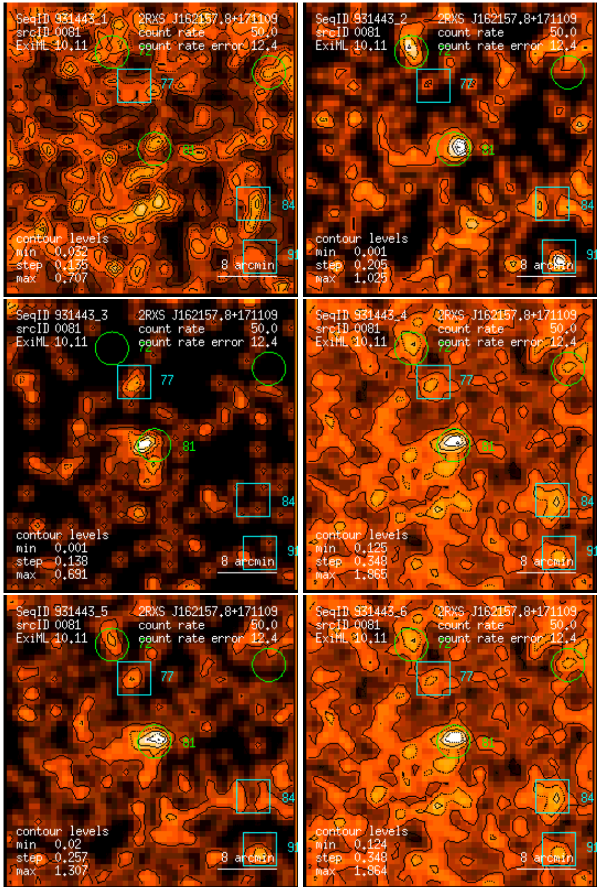
Figure 81: RASS 931443: detection 0081: band rate images, Gaussian filter: (1) PSPC channels 11 – 41, (2) 52 – 90, (3) 91 – 201, (4) 11 – 235, (5) 52 – 201, (6) 11 – 201. Broad band rates in counts/ks. Band rate contour levels in counts/ks/arcmin 2 .
