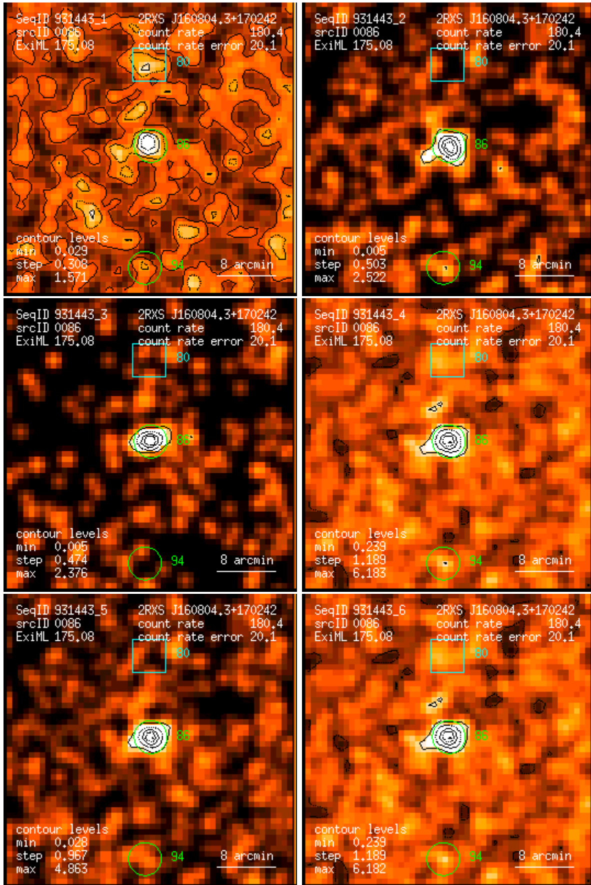
Figure 86: RASS 931443: detection 0086: band rate images, Gaussian filter: (1) PSPC channels 11 – 41, (2) 52 – 90, (3) 91 – 201, (4) 11 – 235, (5) 52 – 201, (6) 11 – 201. Broad band rates in counts/ks. Band rate contour levels in counts/ks/arcmin 2 .
