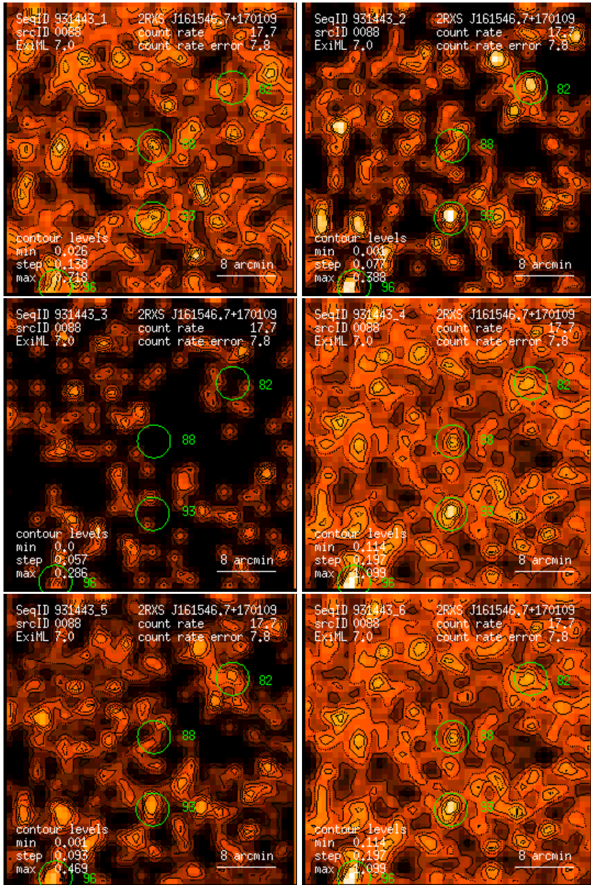
Figure 88: RASS 931443: detection 0088: band rate images, Gaussian filter: (1) PSPC channels 11 – 41, (2) 52 – 90, (3) 91 – 201, (4) 11 – 235, (5) 52 – 201, (6) 11 – 201. Broad band rates in counts/ks. Band rate contour levels in counts/ks/arcmin 2 .
