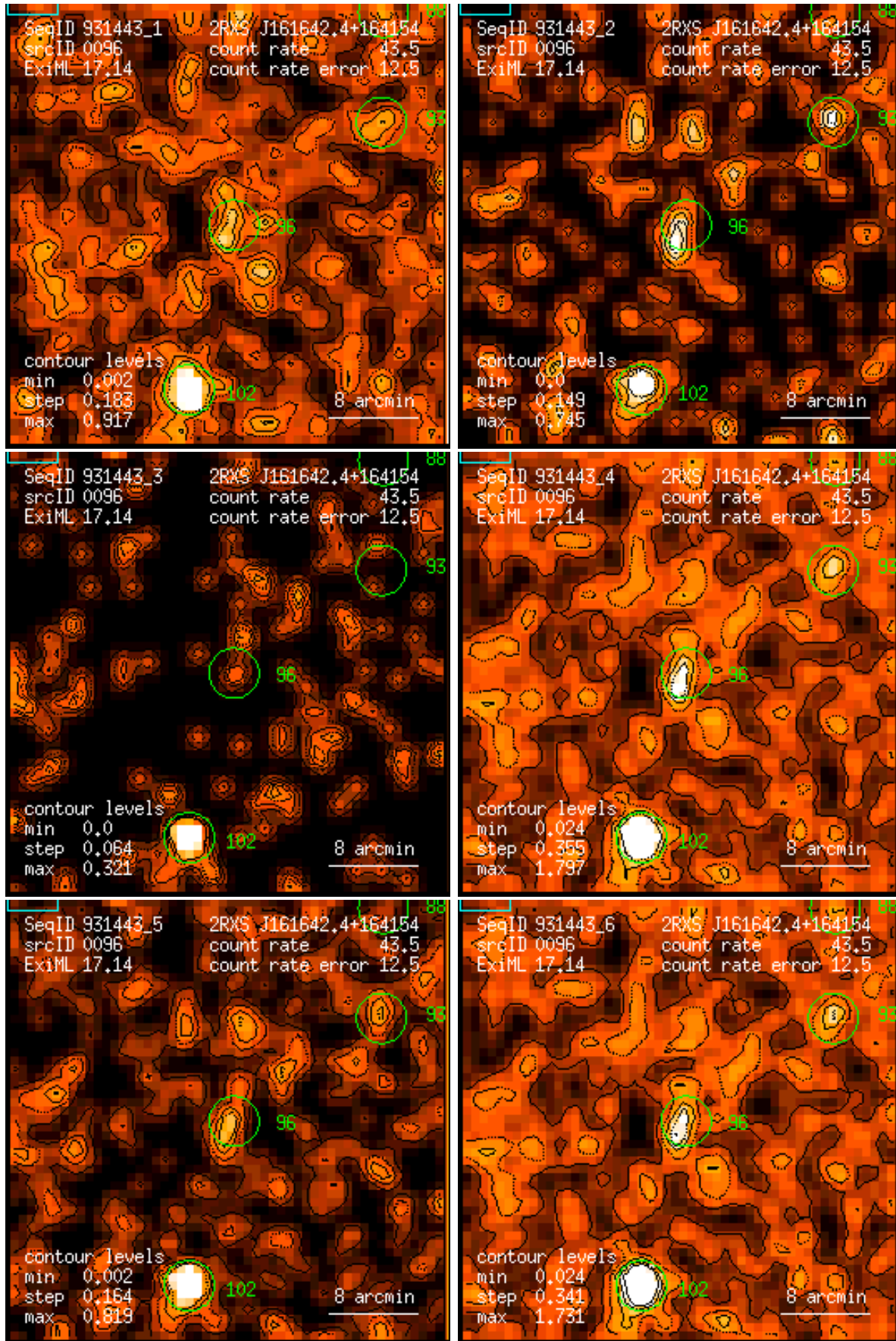
Figure 96: RASS 931443: detection 0096: band rate images, Gaussian filter: (1) PSPC channels 11 – 41, (2) 52 – 90, (3) 91 – 201, (4) 11 – 235, (5) 52 – 201, (6) 11 – 201. Broad band rates in counts/ks. Band rate contour levels in counts/ks/arcmin 2 .
