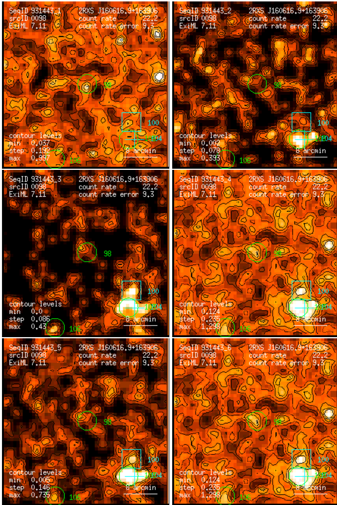
Figure 98: RASS 931443: detection 0098: band rate images, Gaussian filter: (1) PSPC channels 11 – 41, (2) 52 – 90, (3) 91 – 201, (4) 11 – 235, (5) 52 – 201, (6) 11 – 201. Broad band rates in counts/ks. Band rate contour levels in counts/ks/arcmin 2 .
