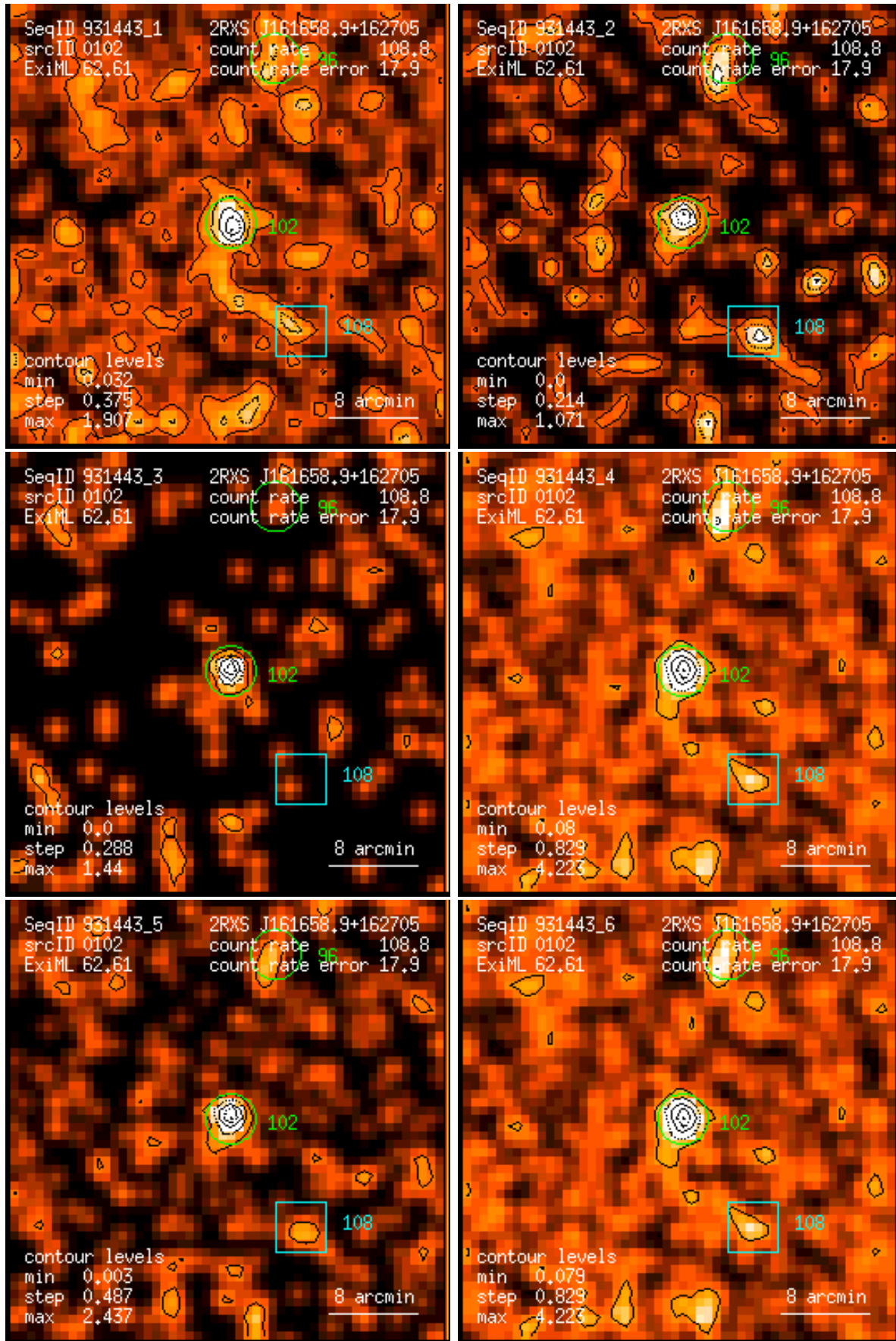
Figure 102: RASS 931443: detection 0102: band rate images, Gaussian filter: (1) PSPC channels 11 – 41, (2) 52 – 90, (3) 91 – 201, (4) 11 – 235, (5) 52 – 201, (6) 11 – 201. Broad band rates in counts/ks. Band rate contour levels in counts/ks/arcmin 2 .
